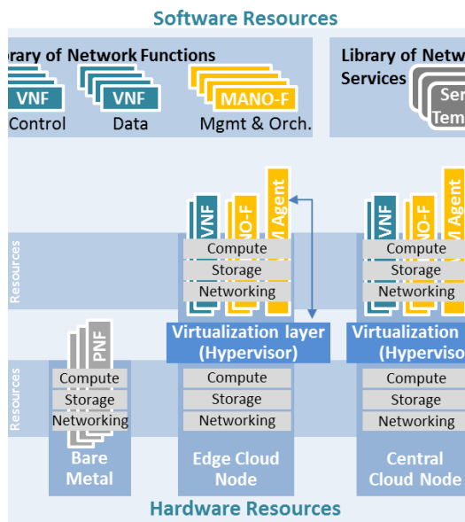
Fig. 4: 5G NORMA Resource view.
