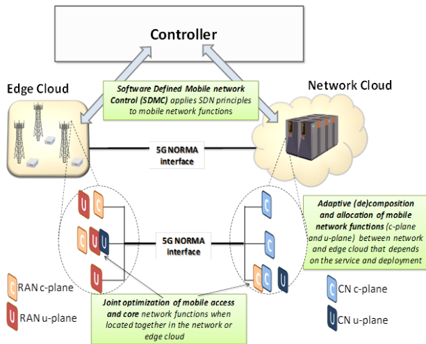
Fig. 2: 5G NORMA concept based on three innovative enablers.
