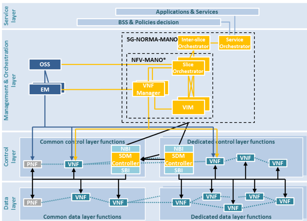
Fig. 3: Preliminary 5G NORMA functional reference architecture.
