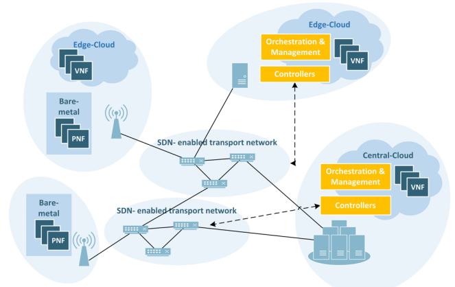
Fig. 6: 5G NORMA Topology view.
