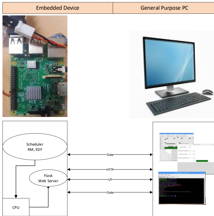
Figure 5. Implementation architecture.
