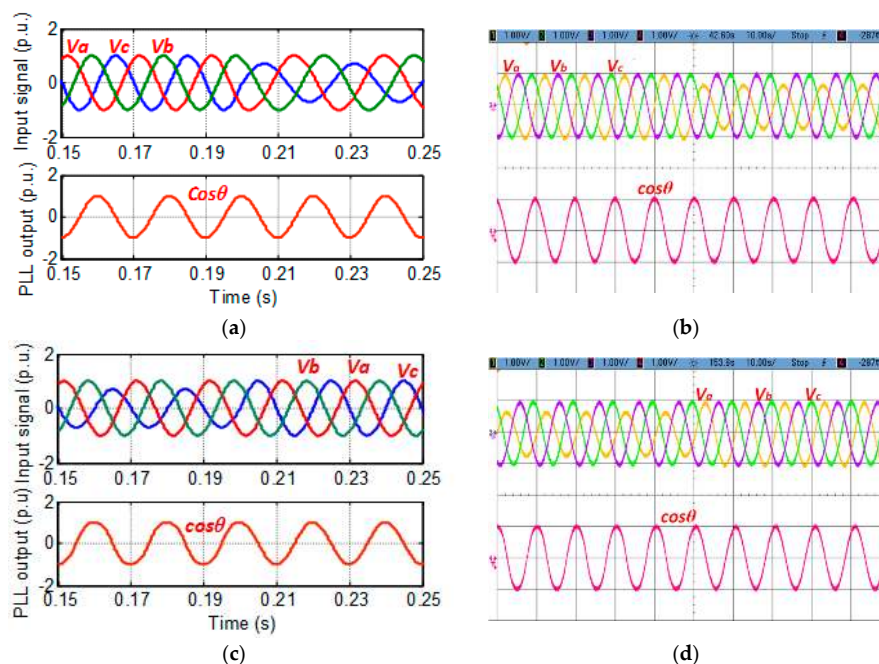
Figure 12. Response of PLL under unbalanced condition: (a) 3- \phi balanced input to 3- \phi unbalanced input (simulation), (b) 3- \phi balanced input to 3- \phi unbalanced input (experimental), (c) 3- \phi unbalanced input to 3- \phi balanced input (simulation), and (d) 3- \phi unbalanced input to 3- \phi balanced input (experimental).
