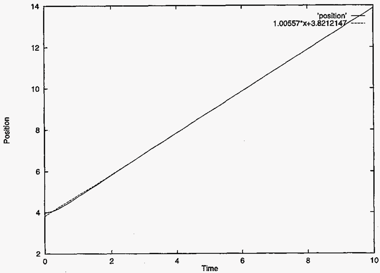
Figure 8: Plot of the center of mass of a rising cap bubble vs. time. We compare this data with the linear best fit for 2 < \text{time} < 10 . Expected slope is 1.
