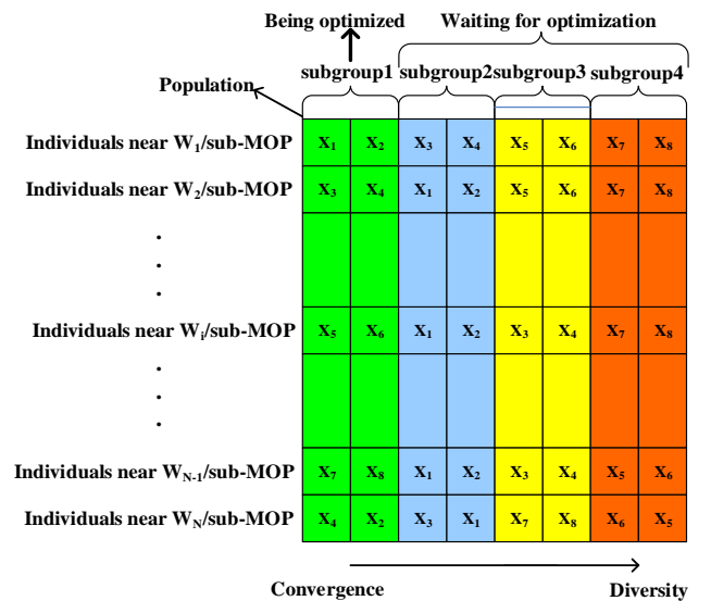
Fig.6. The structure of the population, where the individuals are assigned with different grouped variable sequences.
