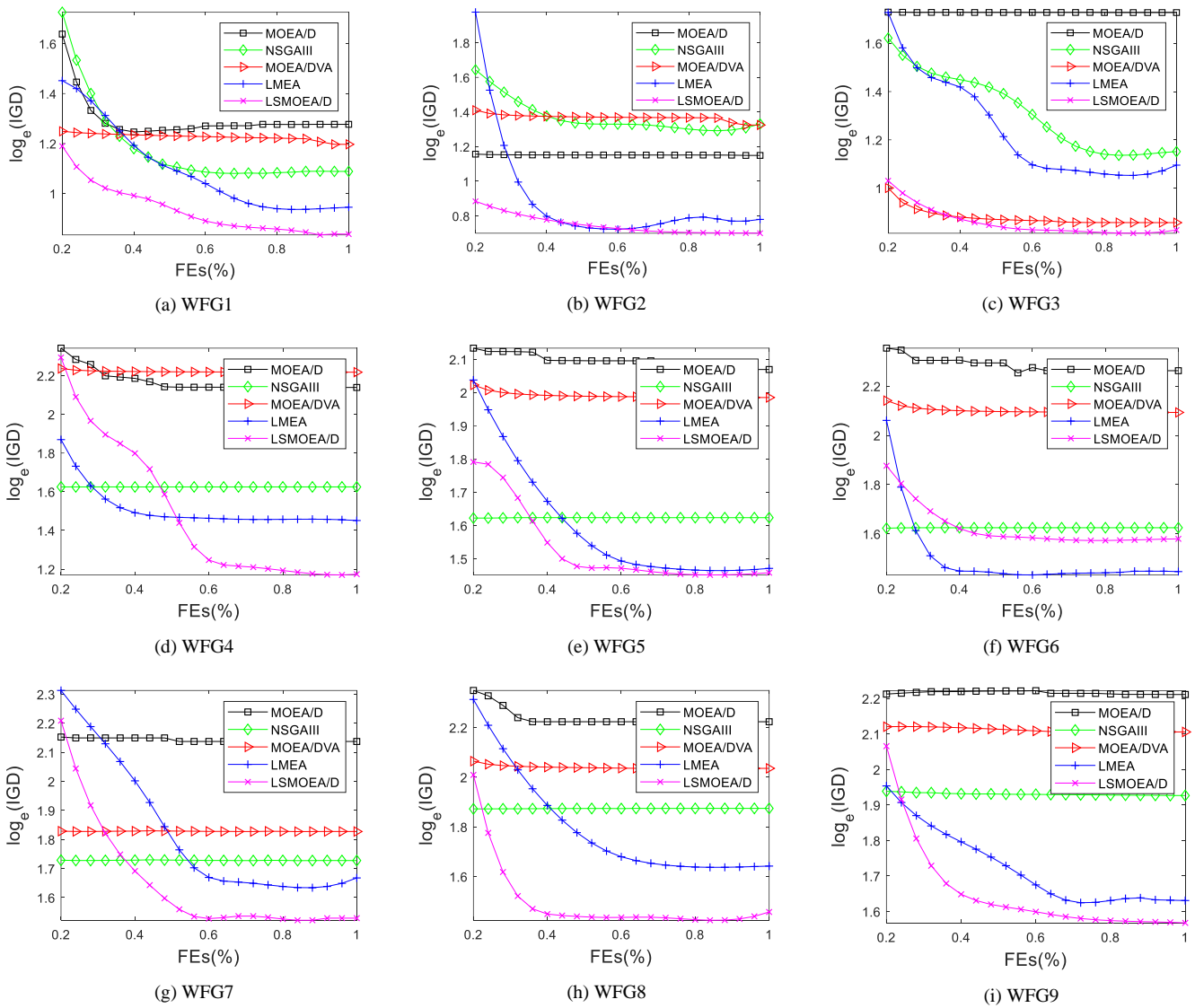
Fig. S5. Evolutionary trajectories of IGD on the 10-objective WFG test problems with 1000 variables. The abscissa is the percentage of consumed FEs.
