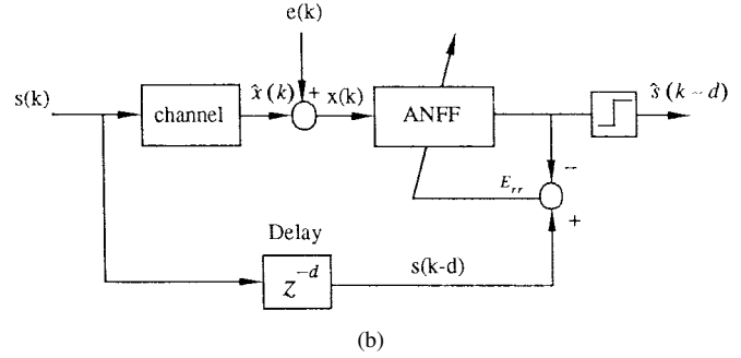
Fig. 7. (a) Schematic of a data transmission system. (b) ANFF as an adaptive equalizer.
