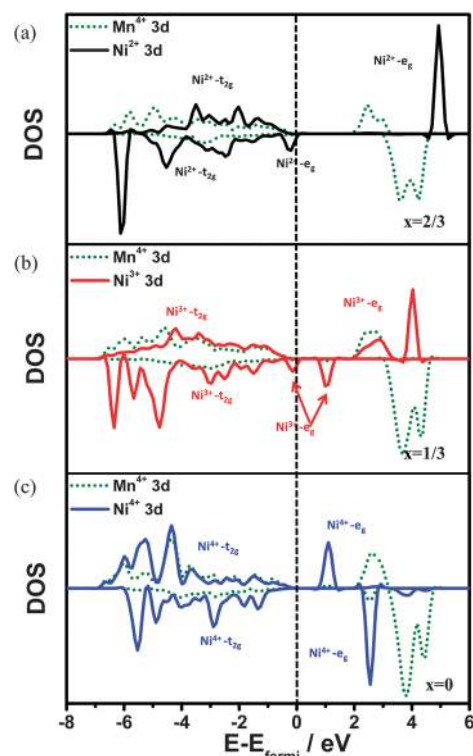
Fig. 5 The electronic structures of Ni 3d and Mn 3d orbitals in \text{Na}_x[\text{Ni}_{1/3}\text{Mn}_{2/3}]\text{O}_2 at (a) x = 2/3 , (b) x = 1/3 , and (c) x = 0 .
