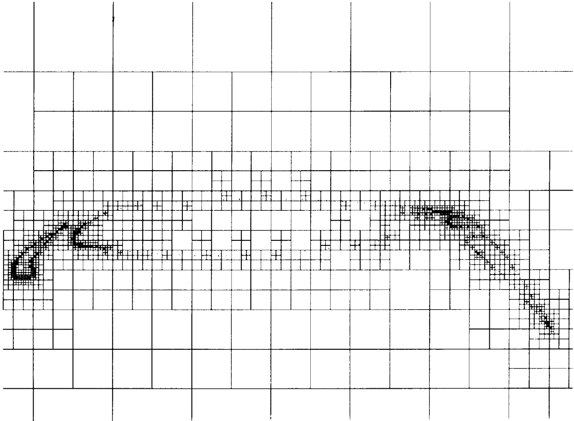
Figure 10 Quadtree Constructed About Initial Boundary Point Distribution This Quadtree is Employed to Support the Background Spacing Function and Also Represents the Initial Form of the Quadtree Employed in the Search for "Close" Front Points.
