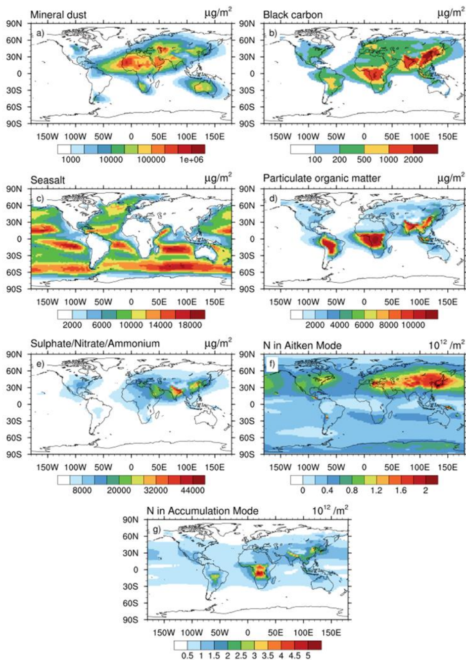
220 Figure 1: Simulated climatological aerosol properties for the lower troposphere (surface to ~700hPa) including vertically integrated mass concentration of mineral dust (a), BC (b), sea salt (c), POM (d), SNA (e), vertically integrated particle number concentration of the Aitken mode N_{\text{akn}} (f) and of the accumulation mode N_{\text{acc}} (g).
