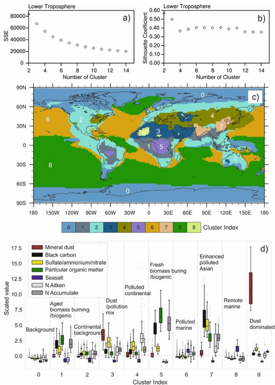
255 Figure 2: Lower troposphere clustering using K-means. The top panel shows the evaluation metrics SSE (a) and SS (b) vs a k range of 2-14. The middle plot (c) highlights the spatial distribution of 10 aerosol regimes for the lower troposphere. The bottom plot (d) 260 shows the data distribution of the 7 considered aerosol properties within the 10 individual aerosol regimes, and cluster names assigned to each cluster based on the analysis of the aerosol data within the respective cluster. The boxplots describe the distribution of data by displaying 5 statistical quantities: the maximum value (top whisker), 75% quantile, median (top of box), median (middle line in box), 25% quantile (bottom of box) and minimum value (bottom whisker) of standardized aerosol parameters that are not outliers. The black dots are outliers which are defined as the data beyond 2.67\sigma of a normal distribution.
