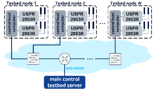
FIGURE 2. Ethernet-based general control system architecture.
