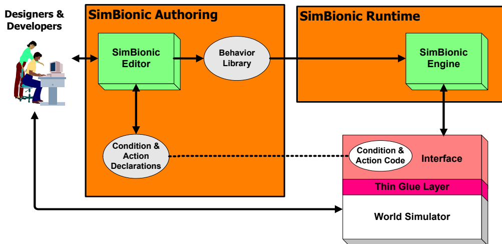
Figure 1- SimBionic Authoring Tool and Engine
