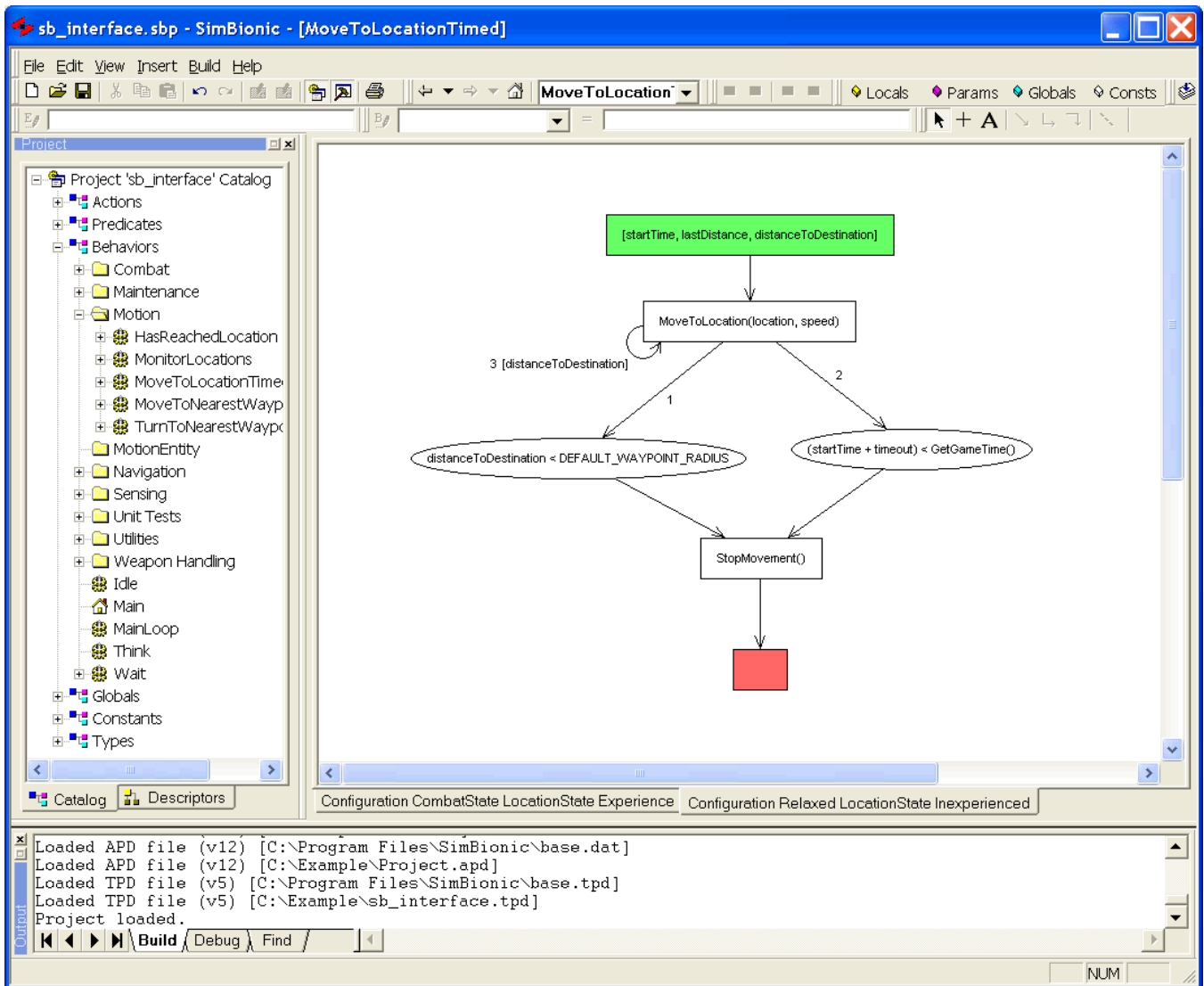
Figure 3- Screenshot of Authoring Tool
