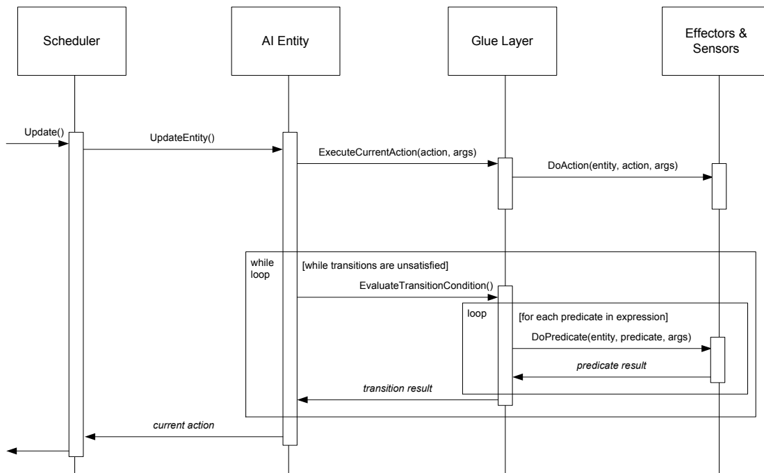
Figure 2- Sequence Diagram of Entity and World Interface
