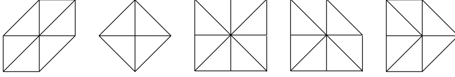
Fig. 1. Examples of patches \Delta_i for d = 2 .
