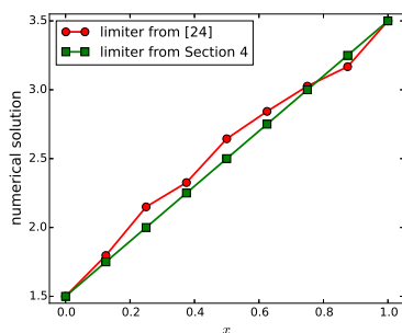
Fig. 6. Example 7.2, cross section of the solutions at y = 0.5 .
