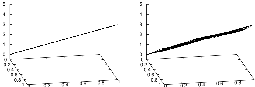
Fig. 5. Example 7.2, solution with the limiter from Sec. 4 (left) and that from Ref. 24 (right).
