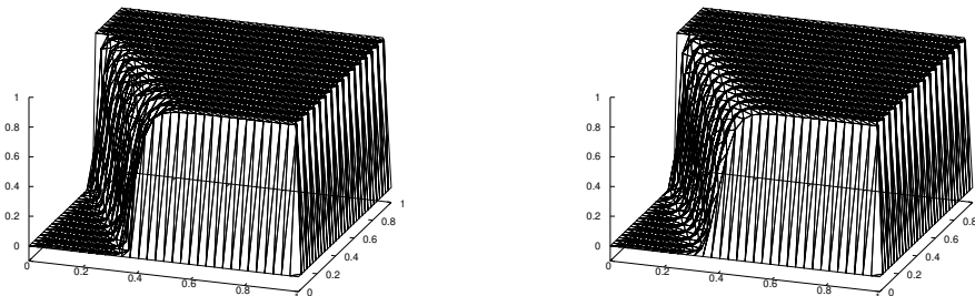
Fig. 7. Example 7.3, solutions obtained with the limiter defined in Sec. 4 (left) and the limiter from Ref. 24 (right).
