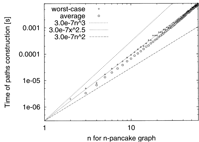
Fig. 9 Time of paths construction.
