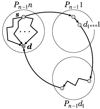
Fig. 3 Case I ( d = d_1 d_2 \dots d_{n-1} n ).
