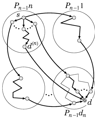
Fig. 4 Case II ( d = n d_2 d_3 \dots d_n, d_n \neq x ).
