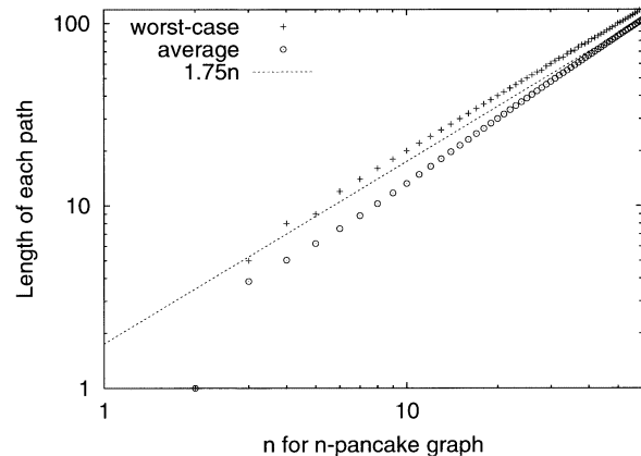
Fig. 8 Length of each path.
