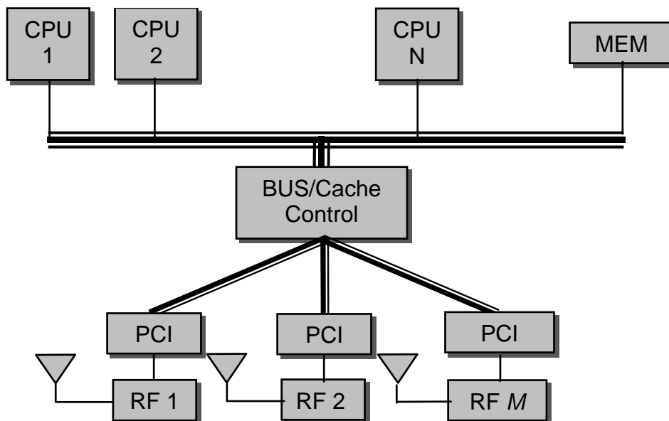
Figure 3: Multi-way SMP Architecture for Radio Gateways
