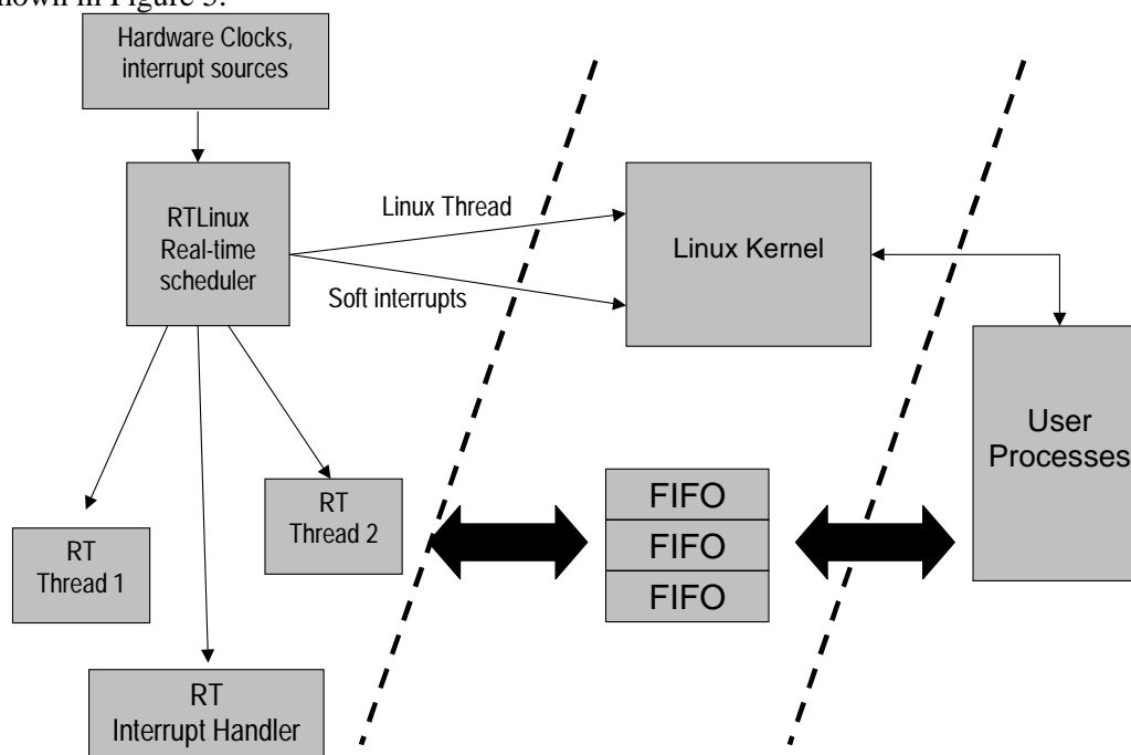
Figure 5: RTLinux Micro-Kernel
