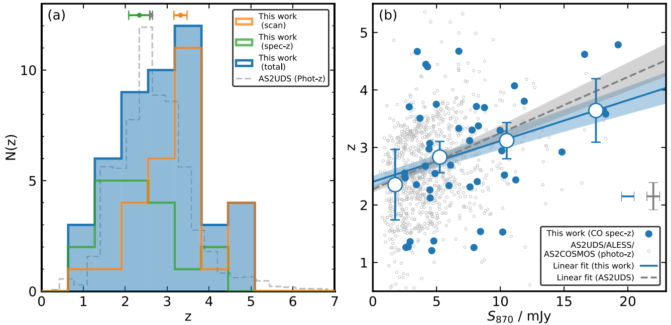
Figure 5. (a) The redshift distribution of our CO sample. We show both the total distribution and the distributions of the scan and spec-z subsamples, and compare these with the photometric redshifts of the AS2UDS sample (scaled for clarity). The medians of each sample are shown by markers at the top of the panel. The submillimetre-bright scan sources generally lie at higher redshifts (median z = 3.32 \pm 0.17 ) than the typically fainter spec-z sample ( z = 2.3 \pm 0.3 ), and the AS2UDS population ( z = 2.61 \pm 0.08 ). (b) Redshift versus 870- \mu\text{m} flux density for our CO sample and the SMGs with photometric redshifts from the AS2COSMOS, AS2UDS, and ALESS surveys (da Cunha et al. 2015; Dudzevičiūtė et al. 2020; Ikarashi et al. in preparation). Our CO sources, binned by S_{870} , are fit with a linear model of increasing redshift with S_{870} , yielding a modest positive correlation with a best-fitting slope of 0.07 \pm 0.01 \text{ mJy}^{-1} . This is consistent with the 0.06 \pm 0.01 \text{ mJy}^{-1} gradient measured by Simpson et al. (2020) for AS2COSMOS and 0.09 \pm 0.02 \text{ mJy}^{-1} measured by Stach et al. (2019) for AS2UDS, supporting the downsizing trend reported by others (see Section 3.2). Representative error bars for our sample and AS2UDS are shown in the bottom right corner of the panel.
