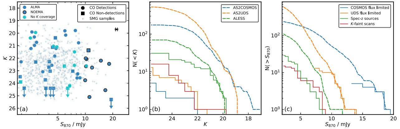
Figure 2. (a) K -band magnitude versus 870- \mu\text{m} flux density for sources targeted in this work (filled), with the parent samples of SMGs from AS2COSMOS, AS2UDS, and ALESS represented by the small points. For our targets, symbol shapes differentiate CO detections from non-detections. ALMA or NOEMA observations are differentiated by the symbol outline. Our sample covers the range of K magnitudes (median K = 22.3 ; 16–84th percentile range 20.7–23.5) spanned by the SMG population, while we typically select sources that are bright at 870 \mu\text{m} (median S_{870} = 5.9 mJy; 16–84th percentile range 2.8–10.5 mJy). 3\sigma upper limits for K non-detections are plotted, and we show a representative error bar for the whole population in the top right corner. Four sources are undetected in the K -band and 14 have no K -band photometry. In the latter cases we estimate K from the typical K - 3.6 \mu\text{m} colour at the appropriate redshift, where IRAC 3.6 \mu\text{m} coverage is available (cyan points). Seven of our targets have no K or IRAC 3.6 \mu\text{m} coverage, and therefore do not appear in this panel. (b): Cumulative histogram of K -band magnitude for our targets compared with their parent samples. Non-detected sources are shown at the relevant 3\sigma flux limit of their respective survey, as for simplicity are the seven sources that are not covered in K or IRAC 3.6 \mu\text{m} . We see that the K - and S_{870} -selected sources mostly sample the K -faint end of the parent sample, whereas the ALESS spec-z sources are complete above K \sim 21 . (c): Cumulative histogram of S_{870} for our targets compared with their parent samples. The S_{870} -selected scan -mode sources are mostly complete above \sim 15 mJy and \sim 10 mJy in AS2COSMOS and AS2UDS, respectively, whereas the K -selected and spec-z sources cover the fainter end of this parameter space.
