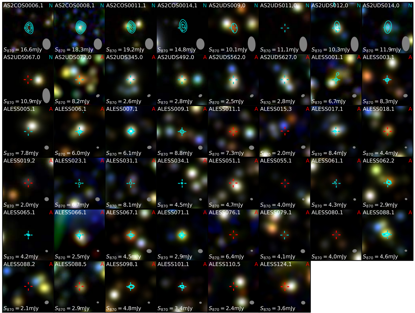
Figure 1. 25 arcsec \times 25 arcsec ( \sim 200 kpc at the median redshift of our sample) colour thumbnails composed of K -band, IRAC 3.6 \mu m and IRAC 4.5 \mu m images of the targets in our sample for which this imaging is available. We see that SMGs are in general redder than field galaxies, but this is not the case for all sources. The crosshair (cyan for CO-detected and red for CO non-detected) indicates the position of the 870- \mu m emission detected by ALMA, with a typical beam size of \sim 0.3–0.5 arcsec, the 870- \mu m flux density of which is reported in each frame. The cyan contours represent CO emission at the 5\sigma , 7\sigma , 9\sigma , and 11\sigma levels. We indicate whether the CO observations of the target come from ALMA (A) or NOEMA (N) and show the synthesised beam in the top- and bottom-right corners, respectively. The ALMA 3-mm beam sizes range between 0.8 arcsec \times 0.6 arcsec and 2.2 arcsec \times 1.8 arcsec, whereas for NOEMA they are typically \sim 6 arcsec \times 4 arcsec.
