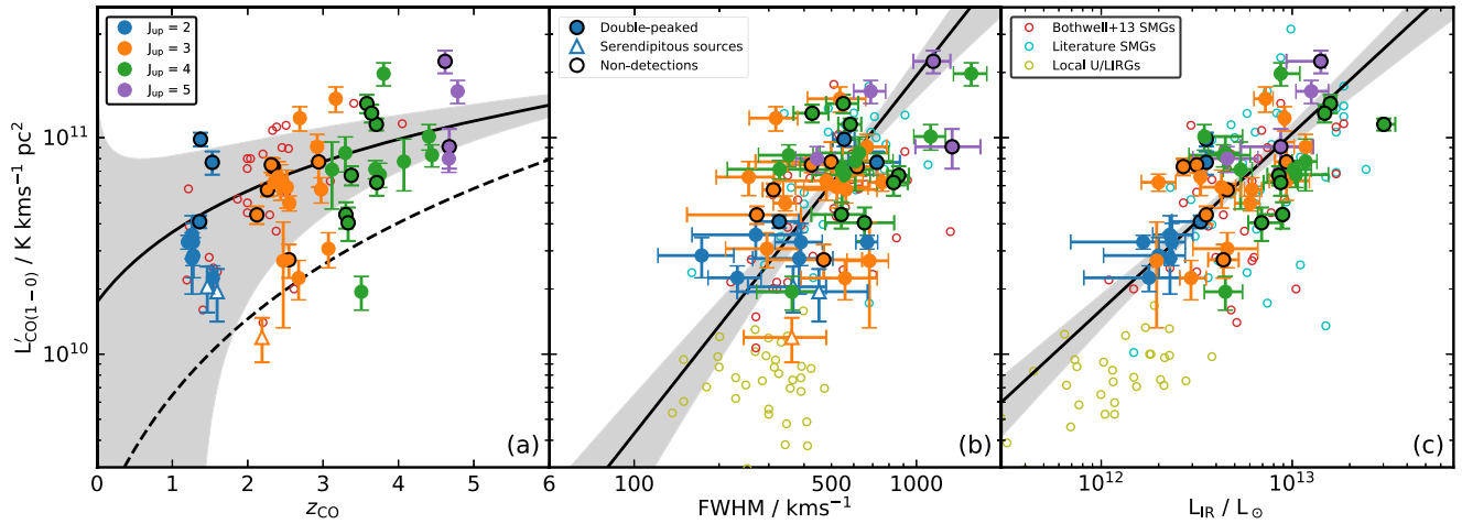
Figure 7. (a) L'_{\text{CO}(1-0)} versus CO redshift for our SMG sample, showing a clear trend of increasing CO luminosity with redshift which we fit with the model L'_{\text{CO}} \propto (1+z)^b , finding b = 1.1 \pm 0.2 . This plot indicates that the gas mass in our dust-mass-selected SMGs exhibits a steady rise with redshift, although this is partly driven by the increase in the sensitivity limit at higher redshifts (roughly indicated by the dashed line as our data have a range of sensitivities). (b) L'_{\text{CO}} versus FWHM for our sample along with SMGs from the literature compilation described in Section 3.3 and local ULIRGs from Downes & Solomon (1998). For our sources, we indicate the transition in which the source was detected, however, all sources have been corrected to L'_{\text{CO}(1-0)} as described in Section 3.3. Most SMGs lie at the high-luminosity end of this trend, with the brightest and broadest lines indicating that they are the most massive galaxies in terms of both gas content and dynamical mass. We generally find that higher J_{\text{up}} sources have larger linewidths, which might suggest that on average the higher redshift sources we detect are more massive. Also included are the three serendipitous sources described in Section 3.1, which lie at the lower end of the trend, suggesting that they may be scaled down versions of SMGs. Our data are fit with the model \log_{10} L'_{\text{CO}} = a \log_{10} (\text{FWHM}/\text{FWHM}_{\text{med}}) + b , with a = 1.7 \pm 0.3 , consistent with a rotating disc model. We also find that the median linewidth of the double-peaked sources is consistent with that of the single-peaked sources, within their 1\sigma uncertainties. ULIRGs display lower line luminosities for a given linewidth, likely because their dynamical masses have an increasing contribution from their stellar component, rather than being dominated by the gas. (c) L'_{\text{CO}} versus L_{\text{IR}} for the same sample as in the middle panel. Again the SMGs lie at the extreme end of the trend, indicating large gas reservoirs and high SFRs. We fit our data with the model \log_{10} L'_{\text{CO}} = a \log_{10} (L_{\text{IR}}/L_{\text{IR,med}}) + b , finding a = 0.82 \pm 0.11 . Our data show a scatter of 0.22 dex around this relation, which is likely driven by the scatter in our CO SLED (see Fig. 6a). We also indicate 3\sigma upper limits on our CO non-detections.
