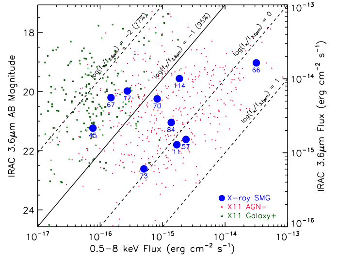
Figure 9. Classification method IV: IRAC 3.6 \mu\text{m} magnitude/flux versus observed-frame 0.5\text{--}8.0 \text{ keV} flux f_{0.5-8\text{keV}} (with no absorption correction). The small red dots and green squares are for the X-ray sources in X11. However, as detailed in Section 4.3, to be conservative, the sources that have z > 1 and were classified as “AGNs” only under the f_{\text{R}}\text{--}f_{0.5-8\text{keV}} criterion in X11 were taken as “Galaxies” here (hence the label “AGN–” and “Galaxy+”). To the lower right of the solid line ( \log(f_{0.5-8\text{keV}}/f_{3.6\mu\text{m}}) > -1 ), 95% of the X11 sources on the plot are AGNs (similarly for the 77% label). Therefore, we choose to classify the SMGs with \log(f_{0.5-8\text{keV}}/f_{3.6\mu\text{m}}) > -1 as AGNs. For X11, sources that are only detected in the soft band or the hard band, the corresponding fluxes in the detection band are used instead of full-band flux upper limits. (A color version of this figure is available in the online journal.)
