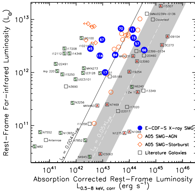
Figure 15. Rest-frame FIR luminosity ( L_{\text{FIR}} ) versus rest-frame 0.5–8.0 keV absorption-corrected luminosity ( L_{0.5-8\text{keV,corr}} ). The large blue dots mark the X-ray detected SMGs in this work with their short LESS IDs in the middle. The small orange open circles (diamonds) are for SMG-AGN (SMG-Starbursts) in A05. The open squares are galaxies whose X-ray and FIR luminosities were calculated by A05 based on data compiled from the literature (see caption of Figure 8 in A05 and references therein). They are classified either as AGN-dominated (labeled with red letter “A”) or star formation-dominated (labeled with green letter “S”) by Rigopoulou et al. (1999) and Tran et al. (2001). The dashed line and gray region is the median luminosity ratio for the quasars in Elvis et al. (1994) and its standard deviation. See Section 7.2.2 for more discussion. (A color version of this figure is available in the online journal.)
