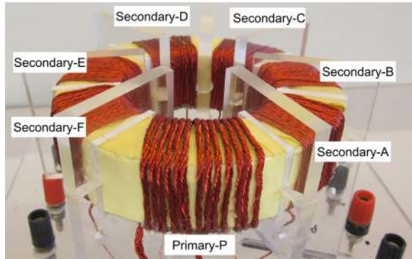
FIG. 1. A photo of the medium frequency magnetic-link.
