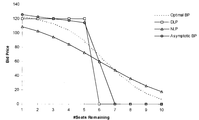
Figure 2 Bid Prices for Example 2
