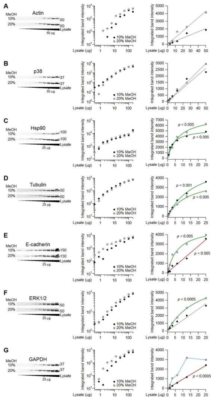
Fig. 4. Linearity and hyperbolic saturation of immunoblots determined by serial dilution. ( A and B ) Immunoblots for actin and p38 are linear under both transfer conditions. ( C and D ) Immunoblots for Hsp90 and tubulin are hyperbolicly saturated under both transfer conditions. ( E to G ) Linear detection of immunoblots for E-cadherin, ERK1/2, and GAPDH occurred with tank transfer conditions containing 10% methanol. HT-29 cells were lysed in RIPA buffer, immunoblotted for the indicated targets, and imaged. Left panels show the immunoblots, middle panels show log-log plots of the quantified band intensities from the
