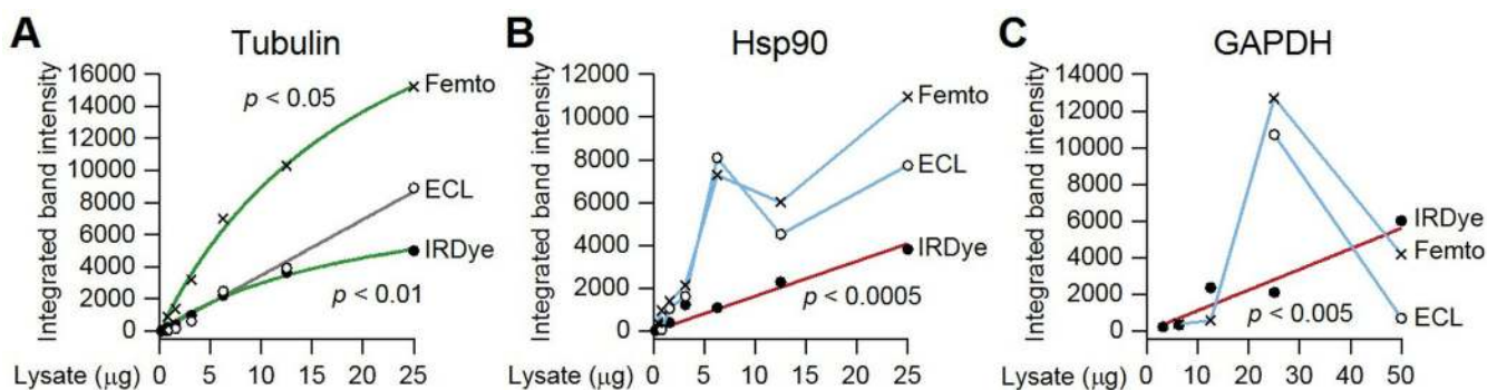
Fig. 5. Quantitative immunoblotting is challenging when imaging by chemiluminescence. (A to C) HT-29 lysates were prepared as in Fig. 4, immunoblotted for the indicated proteins, and imaged by IRDye fluorescence, enhanced chemiluminescence (ECL), or SuperSignal West Femto chemiluminescence as described (12, 16, 45, 46). Linear fits are shown in gray when the hyperbolic model is not significantly better than the linear model for that imaging condition. Linear fits are shown in red when the linear fit of the associated imaging condition is significantly better than the linear fit of the other imaging conditions. Hyperbolic fits are shown in green when the hyperbolic model is significantly better than the linear model for that imaging condition. Data are interpolated in blue when neither the linear nor the hyperbolic model provides a better fit. All model comparisons were done by the F test at a false-discovery rate of 5% ( n = 4–8 dilutions). See file S2 for raw images and calculations.
