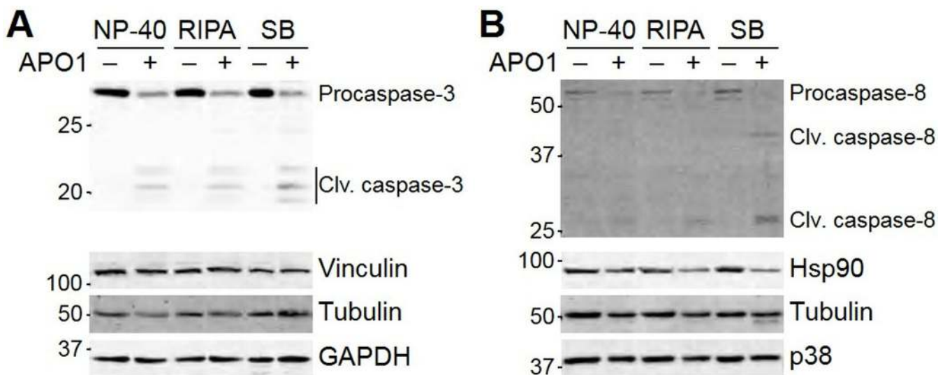
Fig. 2. Posttranslational modifications can move protein into the insoluble fraction of common lysis buffers. MCF10A-5E cells were exposed to the Fas crosslinking agent anti-APO-1 (1 µg/ml) (48) for 24 hours, then floating and adherent cells were lysed in NP-40 lysis buffer, RIPA buffer, or dithiothreitol-containing Laemmli sample buffer (SB). (A) Effect of solubilization conditions on the detection of cleavage products of caspase-3. (B) Effect of solubilization conditions on the detection of cleavage products of caspase-8. Vinculin, tubulin, GAPDH, Hsp90, and p38 were used as loading controls where indicated. Data are representative of three experiments.
