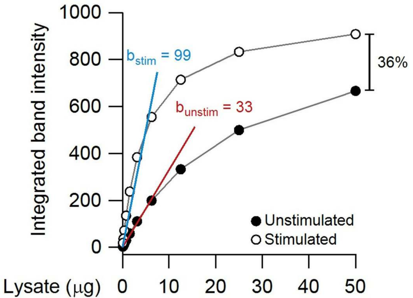
Fig. 9. Quantifying partially saturated immunoblots can dramatically underestimate differences between samples. In this theoretical example, a serial dilution is performed with unstimulated and stimulated extracts. The relative change in the linear range of the immunoblot is 99 (blue) / 33 (red) ~ threefold, whereas the relative change at fivefold higher loading is only 1.4 fold (36%).
