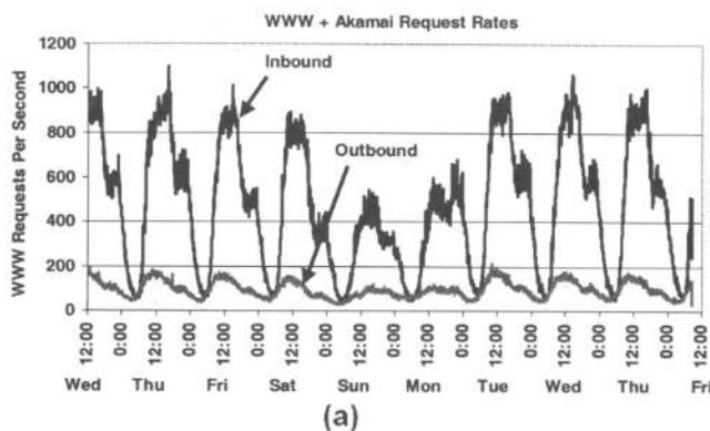
Figure 8. Request rates over time: inbound and outbound HTTP transaction rates for (a) the WWWW + Akamai, and (b) Kazaa.
