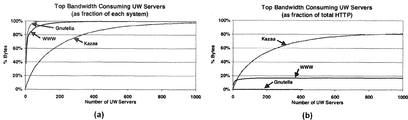
Figure 10. Top UW-internal bandwidth producing servers: a CDF of bytes produced by the top 1000 bandwidth-producing UW-internal servers (a) as a fraction of each system, and (b) as a fraction of the total HTTP traffic.
