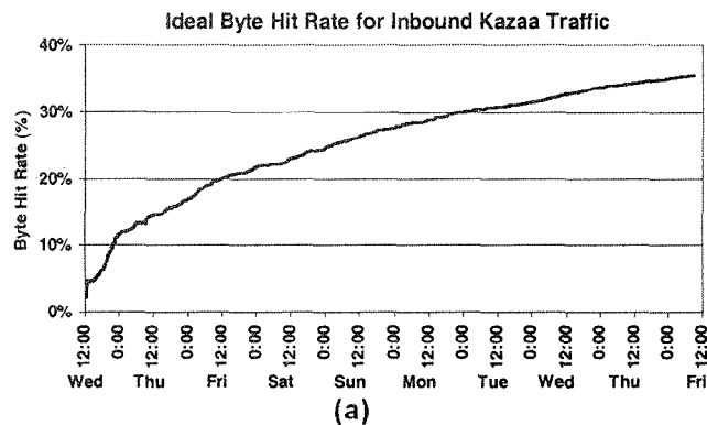
Figure 14. Ideal Kazaa cache byte hit rate: cache byte hit rate over time, for (a) inbound traffic (requests from UW clients) and (b) outbound traffic (requests from external clients).
