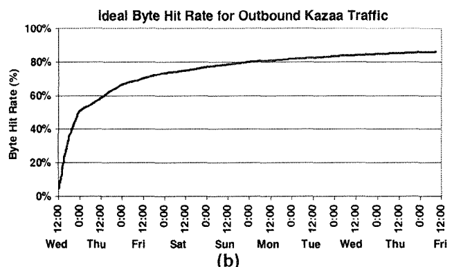
Figure 14. Ideal Kazaa cache byte hit rate: cache byte hit rate over time, for (a) inbound traffic (requests from UW clients) and (b) outbound traffic (requests from external clients).
