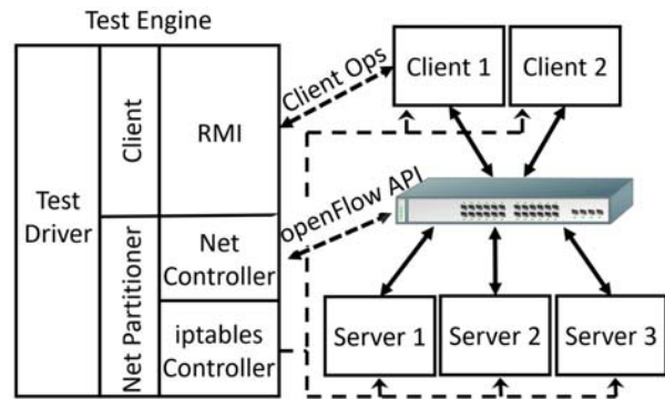
Figure 2. NEAT architecture.
