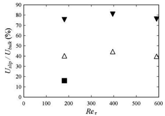
FIG. 16. Slip velocity as a percentage of bulk velocity for g/w=1 , w/H=g/H=0.18750 ridges ( \Delta ) and g/w=3 , w/H=0.09375 , and g/H=0.28124 posts ( \blacktriangledown ) at Re_\tau \approx 180, 395 , and 590 , as well as transverse g/w=1 , w/H=g/H=0.18750 ridges ( \blacksquare ). Note that the ridge spacing in wall units increases with increased Re_\tau .
