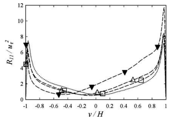
FIG. 21. Re_\tau \approx 395 . R_{11} profiles from simulations with w^+=g^+=37.031 ( \square ) and w^+=g^+=74.062 ( \Delta ) ridges, as well as w^+=37.031, g^+=111.09 ( \blacktriangledown ) posts. Regular channel profile ( \cdots ) shown for reference. Note that symbols are used to identify curves, and do not reflect data point locations.
