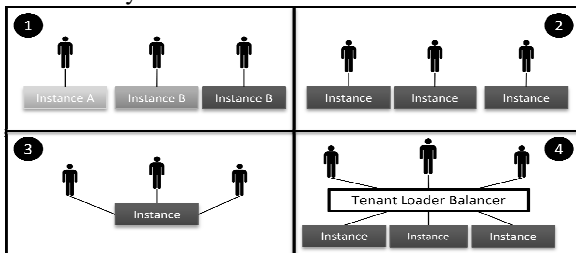
Figure 2: Multi-tenancy approaches [13]
