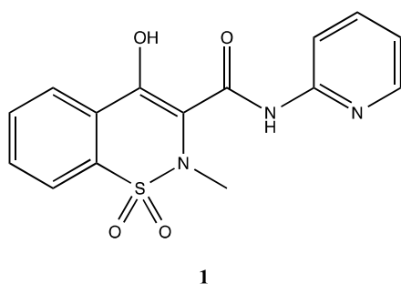
4-Hydroxy-2-methyl-N-(2-pyridinyl)-2H-1,2-benzothiazine-3-carboxamide 1,1-dioxide (Piroxicam)
