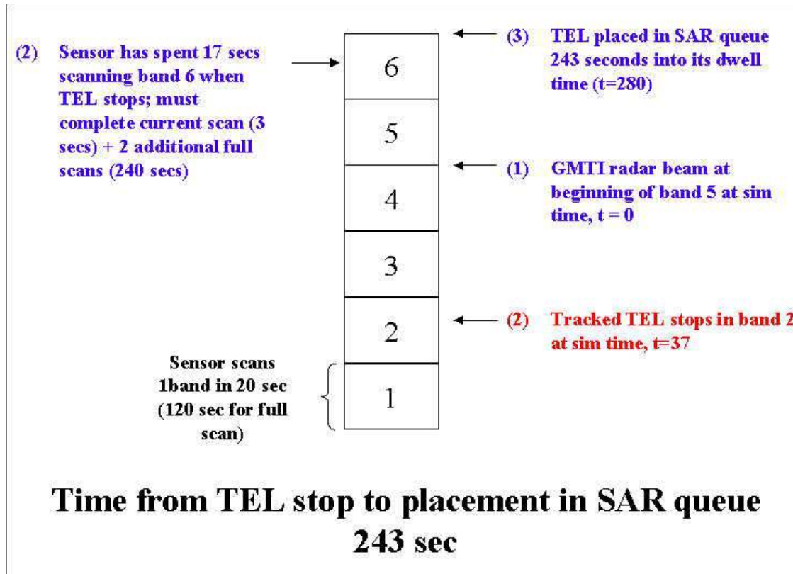
FIGURE 4. TIME TO DETECT A STOPPED TEL. THE BLOCKS LABELED ONE THROUGH SIX REPRESENT THE GMTI SENSOR BANDS. IN THIS CASE, THE TEL STOPS AFTER THE SENSOR HAS PASSED OVER ITS LOCATION DURING THE CURRENT GMTI SCAN.
