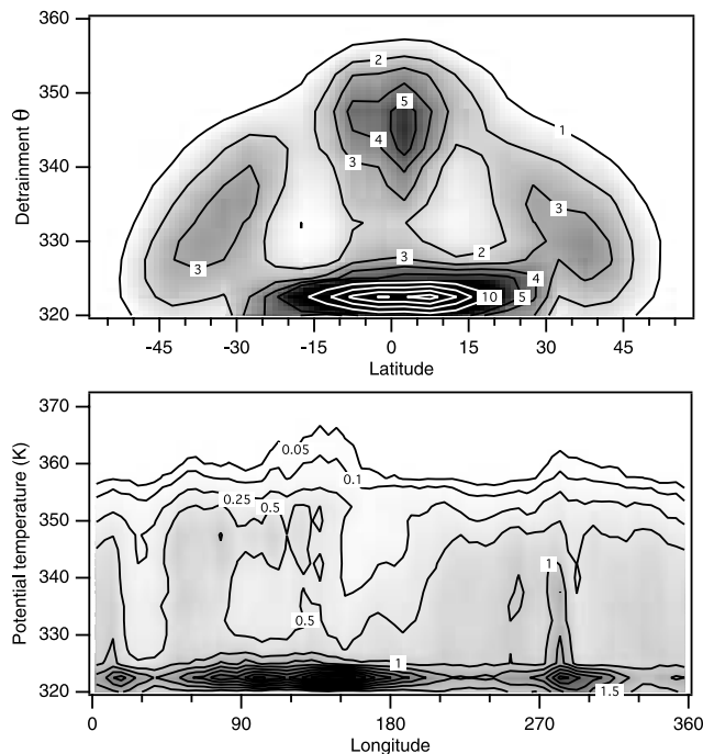
Figure 3. Two-dimensional probability distribution (in 10^{-2}\% ) of dehydration location versus detrainment \theta , based on the set of trajectories initialized at 547 hPa ( \sim 322\text{-K } \theta ). The top plot is versus latitude; the bottom plot is versus longitude. The figures are shaded to improve readability. In the top plot, white contours have values greater than 10, and their contour interval is 5.
