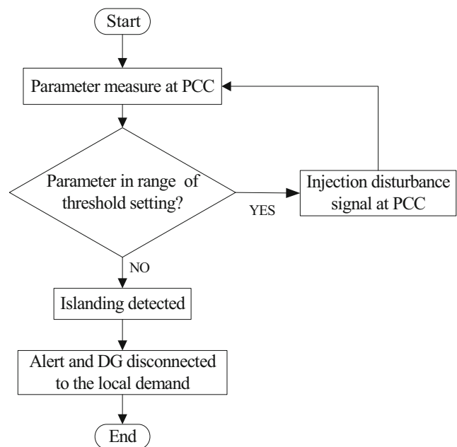
Fig. 8 Flow chart describing the process of a hybrid islanding detection procedure
