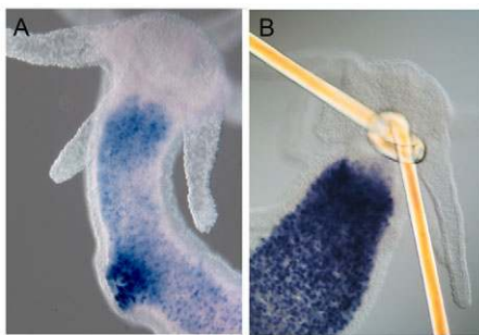
Fig. 5. hydck1/2/4 -expression dynamics. (A,B) hydck1/2/4 -expression dynamics in injured (A) and ligated (B) animals after 6 hours and 1 hour, respectively.
