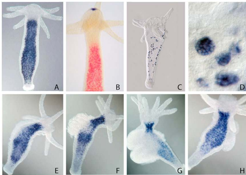
Fig. 3. hydkk1/2/4 -expression analysis by whole-mount in situ hybridization. (A) Whole animal. (B) Double ISH: hywnt3a (blue) and hydkk1/2/4 (red). (C, D) Residual gland cells in epithelial animals of strain sf-1 after heat shock; individual gland cells are shown in D. (E-H) Animals undergoing gametogenesis. (E-G) Oogenesis; (H) spermatogenesis.
