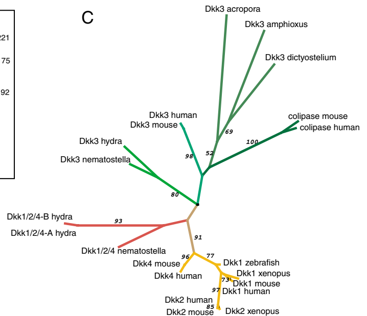
Fig. 2. Sequence analysis of hydkk1/2/4 . (A) TCooffee alignment of HyDkk1/2/4 with the CRD2 of available Dkk molecules (see Materials and methods). (B) Domain structure of mouse Dkk4, NvDkk1/2/4 and HyDkk1/2/4; shaded boxes indicate conserved residues within CRD2; cysteines in red. (C) IQPNNI ML tree of Dkk CRD2 domains with TREE-PUZZLE support values (>50).
