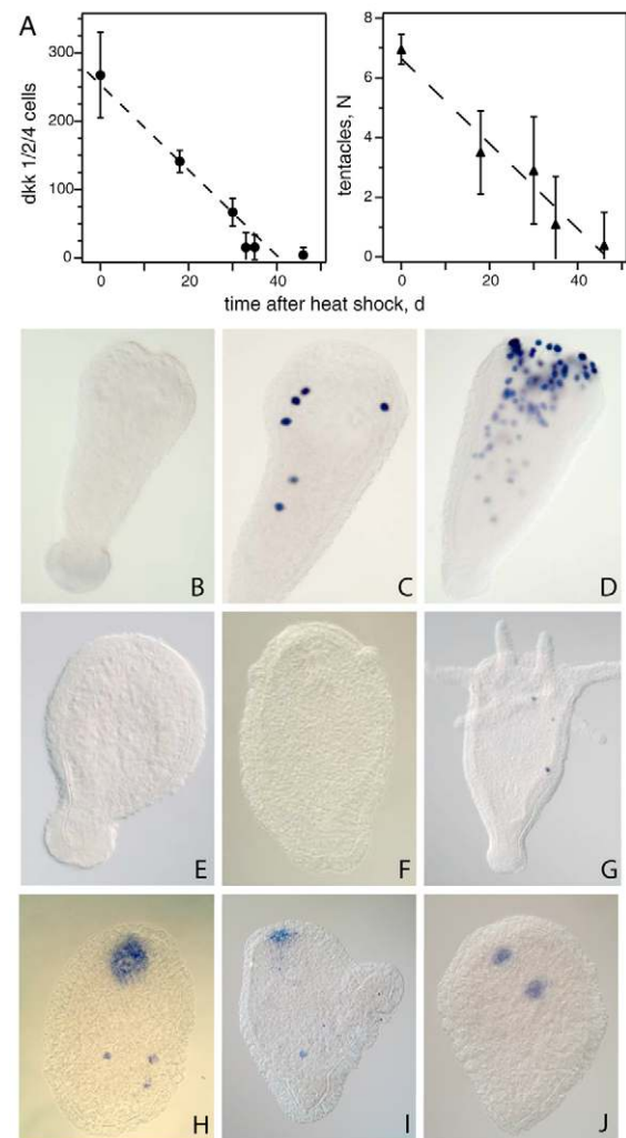
Fig. 6. hydck1/2/4 and hywnt3a expression in regenerating epithelial sf-1 polyps. (A) Quantification of residual hydck1/2/4 -positive gland cells in body column pieces (left); n=6, 3, 5, 48, 37 and 22 with increasing time. Efficiency of head regeneration was measured as the average number of tentacles per regenerate (right); n=20, 101, 69, 178 and 140 . Bars indicate s.d. Animals were cut at 50% body length and regenerated at least 4 hours prior to in situ hybridization and up to 9 days for determination of regeneration behaviour. (B-G) hydck1/2/4 expression in individual regenerates, 4 hours (B-D) and 9 days (E-G) after head removal. (H-J) Ectopic hywnt3a expression in regenerating epithelial sf-1 polyps (5-9 days regeneration).
