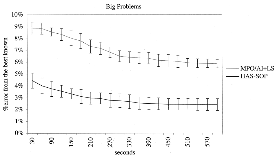
Figure 13. Comparison between MPO/AI+LS and HAS-SOP over big problems. Results are obtained over five runs of 600 seconds. Error bars (one standard deviation) are shown.
