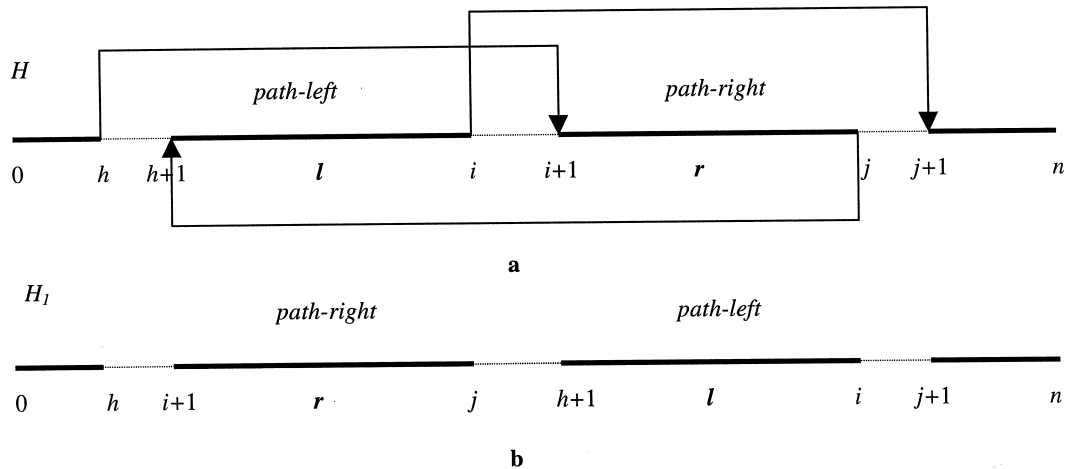
Figure 5. A path-preserving-3-exchange.
