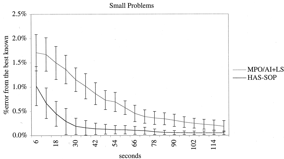
Figure 12. Comparison between MPO/AI+LS and HAS-SOP over small problems. Results are obtained over five runs of 120 seconds. Error bars (one standard deviation) are shown.
