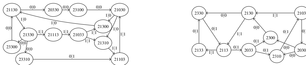
(b) \mathcal{T}_B corresponds to \mathcal{T}_A when unused transitions are deleted.
