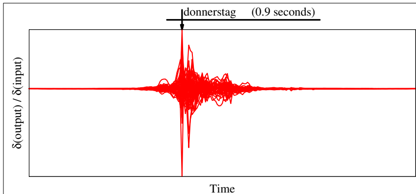
Fig. 2. Example of network outputs dependency with respect to the inputs. The figure shows the dependency of the output unit associated with keyword “donnerstag” at the time step when this keyword is detected in figure 1, with respect to the network inputs at various time steps around the detection point (indicated by an arrow at the top of the figure). In addition, the extent (0.9s) and location of the keyword in the speech signal is shown at the top of the figure. As can be seen, the probability of detecting the keyword depends on the inputs over a long time span, and decreases towards the end of the keyword which is the least discriminative part of it: “tag” (day).
