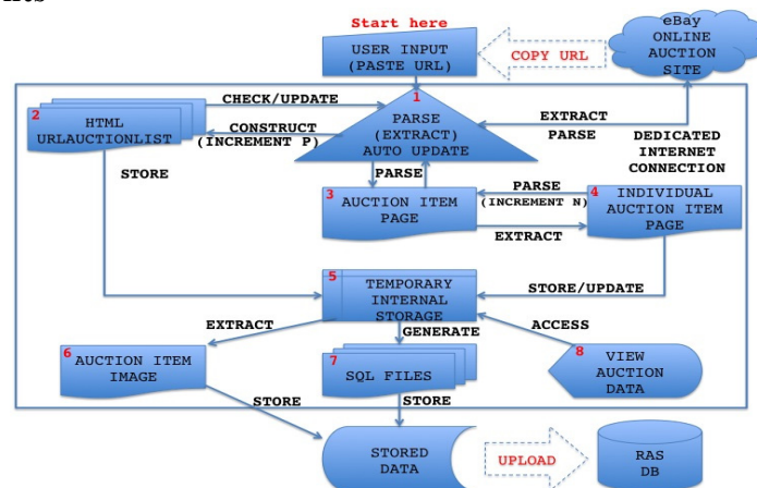
Fig. 3: The internal architecture of the application tool.
