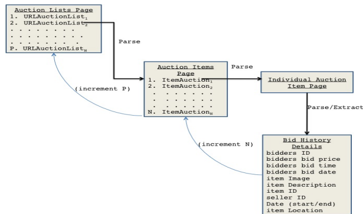
Fig. 2: The process involved with collecting data from an online auction source.
