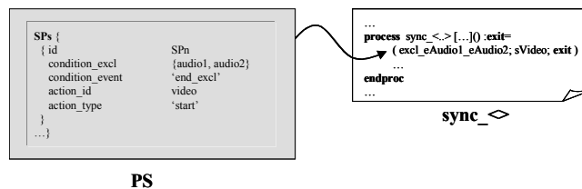
Figure 18. Translation of a synchronization point into a sync_behavior
