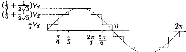
Fig. 4. Synthesized ac voltage v_L of the double-series three-phase twelve-pulse diode rectifier without commutation capacitor.
