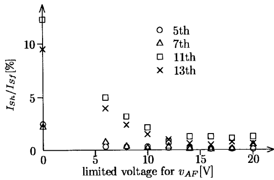
Fig. 14. Experimental results of relationships between voltage limitation of v_{AF} and supply current harmonics.
