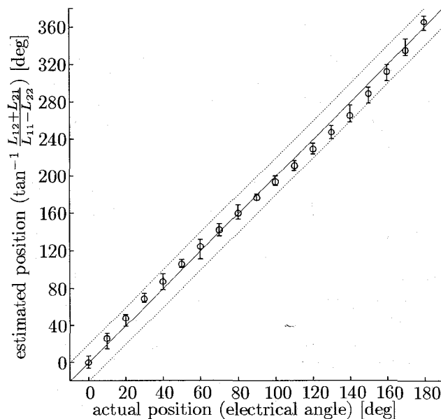
Fig. 8. Experimental result at standstill.
