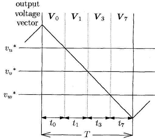
(a) comparing voltage references with triangle
