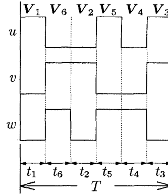
(a) PWM pattern
