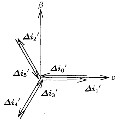
(c) Trajectory of harmonic current vectors
