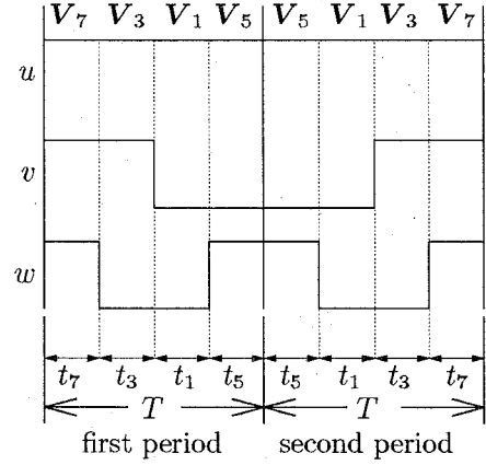
(a) PWM pattern
