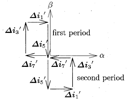
(c) trajectory of harmonic current vector
