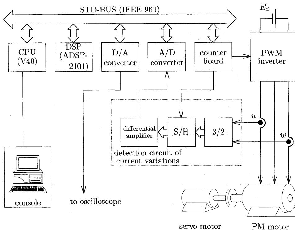
Fig. 7. Configuration of experimental system.
