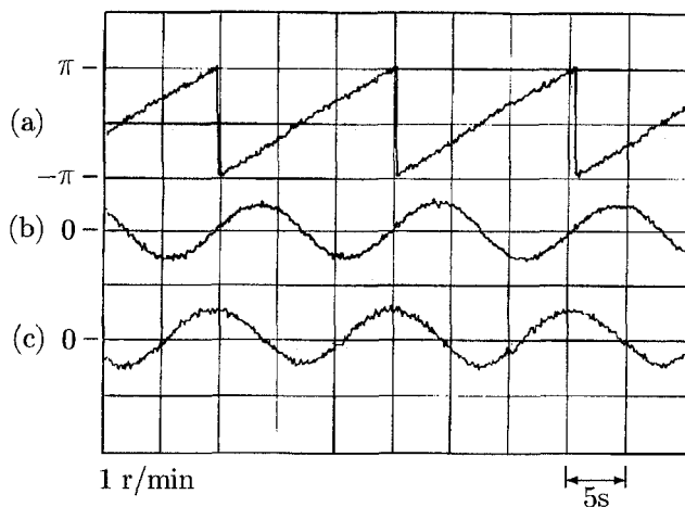
Fig. 9. Experimental result at 1 r/min. (a) estimated position \tan^{-1} \frac{L_{12}+L_{21}}{L_{11}-L_{22}} . (b) L_{12} + L_{21} . (c) L_{11} - L_{22} .
