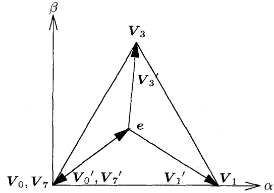
(b) voltage vectors
