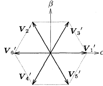
(b) Trajectory of harmonic current vectors
