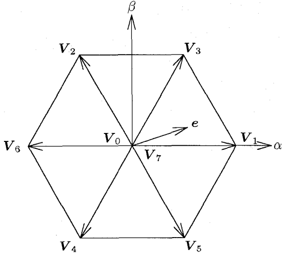
Fig. 2. Voltage vectors of inverter output.
