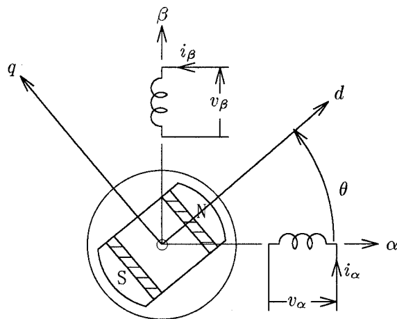
Fig. 1. Model of salient PM motor.
