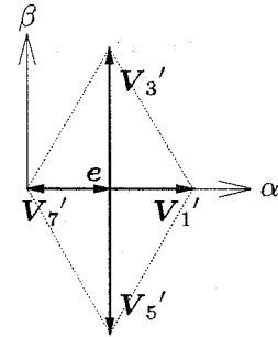
(b) harmonic voltage vectors
