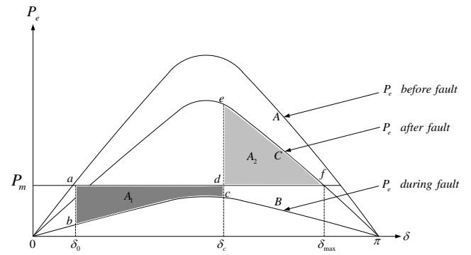
Figure 4. EAC for critical clearing angle
