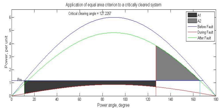
Figure 6. Equal area criterion for Bakuru Hydro Plant
