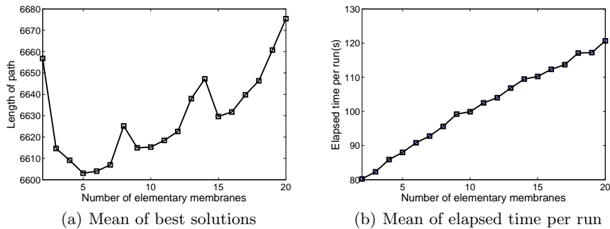
Fig. 12. Experimental results of Ch150 with different membranes
