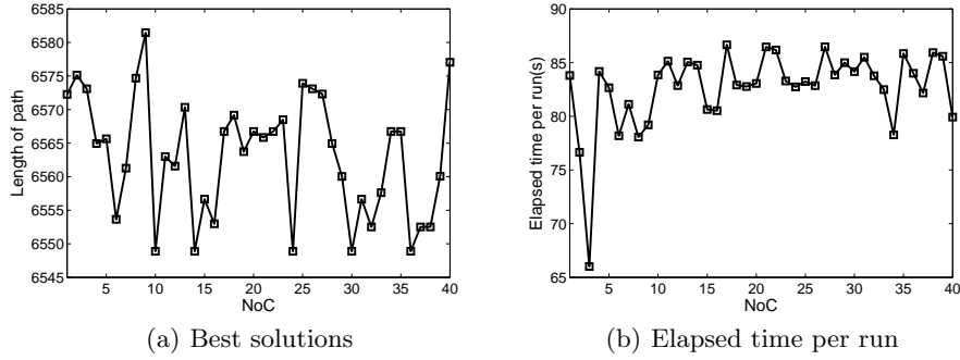
Fig. 19. Experimental results of Ch150 with NoC
