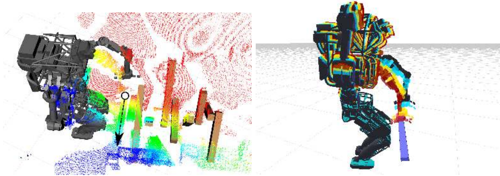
Figure 11: A fitting algorithm produces an affittance that can be used to plan a reach motion. Left: A line annotation defines a search region that is used by a segmentation algorithm to fit a 2"x4" board affittance to the 3D point cloud data. Right: An end-effector goal placed on the board affittance is used to compute a reaching plan.
