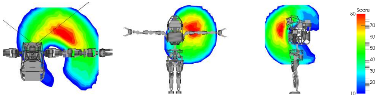
Figure 2: Visualization of the kinematic reachability of the robot from inferior (left), anterior (center), and medial (right) perspectives. We uniformly sampled 15 angles in the feasible range of each of the 6 right arm joints, divided the reachable workspace into 20 \times 20 \times 20 bins, and assigned each bin a score based on how many distinct end-effector orientations it contained.
