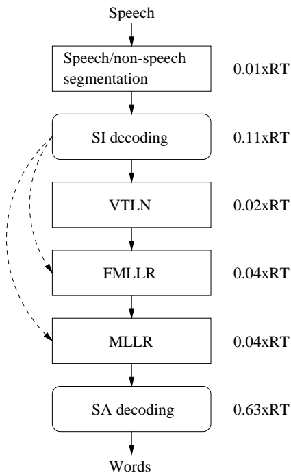
Figure 1: System diagram. Dashed lines indicate that the FMLLR and MLLR steps rely on the 1-best output of the speaker independent decoding. Runtimes are reported on a Linux Pentium 4 3.0GHz, 1.0Gb machine and are exclusive of the feature computation and various data motion steps (which together account for 0.12 \times RT ).
