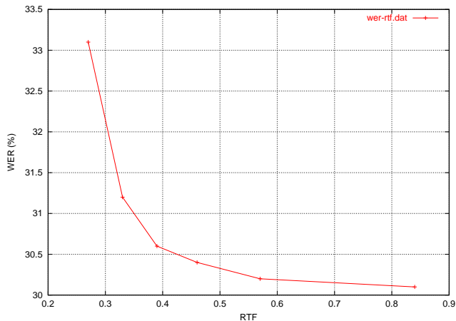
Figure 2: Word error rate versus real-time factor for the speaker-adapted decoding on the RT'02 test data.
