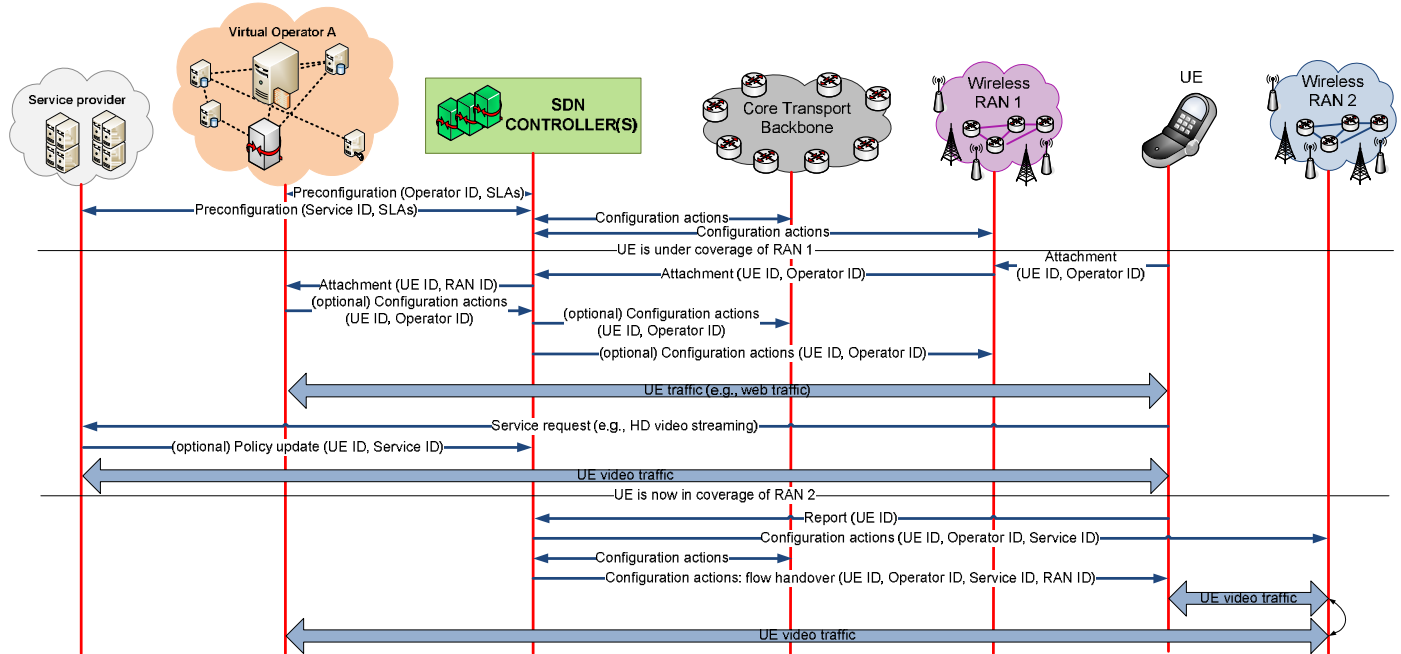
Figure 4. Case study: SDWN high-level interactions
