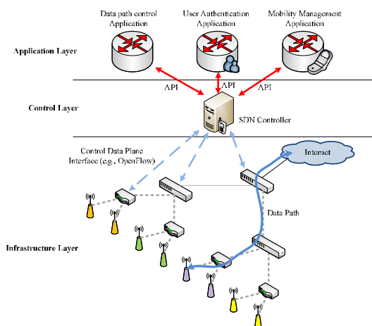
Figure 1. SDN reference architecture
