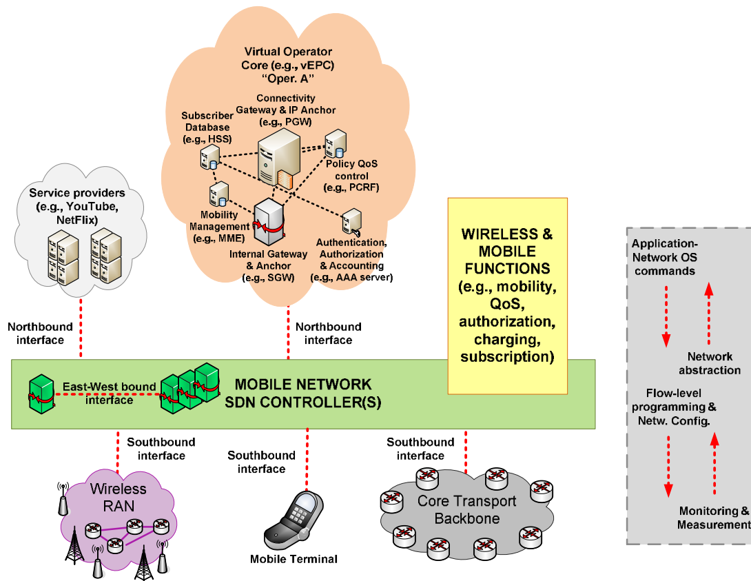
Figure 3. SDN-based mobile network interface architecture
