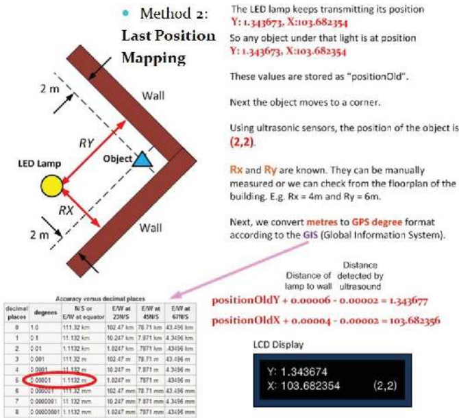
Fig. 3. Determining receiver position using last position method.
