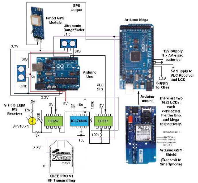
Fig. 5. Circuit diagram of the outdoor-indoor positioning receiver. The XBee Pro transceiver is optional. A GSM module would be enough for most applications and it is more reliable.
