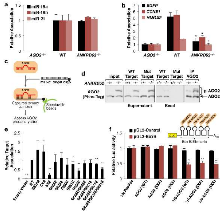
Fig. 3. AGO2 phosphorylation impairs mRNA target association
