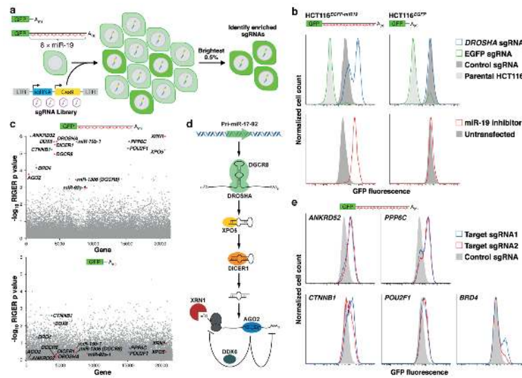
Fig. 1. A genome-wide CRISPR-Cas9 screen reveals known and novel regulators of the miRNA pathway
