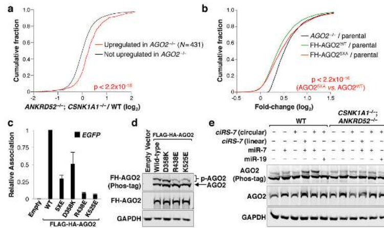
Fig. 5. Argonaute S824-S834 phosphorylation is required for fully efficient miRNA-mediated silencing and is triggered by target binding
