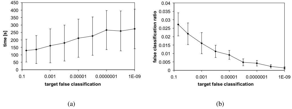
Fig. 3. (a) Time until correct classification of misbehaving nodes and (b) false classification ratio versus target false positive classification probability \alpha .
