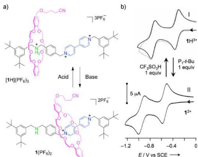
Figure 2. a) Acid–base-controlled ring shuttling in the bistable rotaxane 1H^{3+}/1^{2+} . b) Cyclic voltammogram (acetone/TBAPF 6 , 400 μM, 300 mVs -1 ) of 1H^{3+} (I, full line) and of its deprotonated form 1^{2+} (II), obtained upon addition of one equivalent of P 1 -tBu. The successive addition of triflic acid in stoichiometric amount regenerates 1H^{3+} (I, dashed line).
