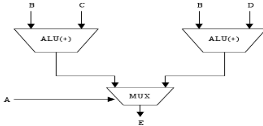
Figure 8: Bad resource allocation
