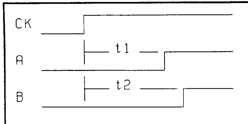
Figure 18 : Waveform 1
