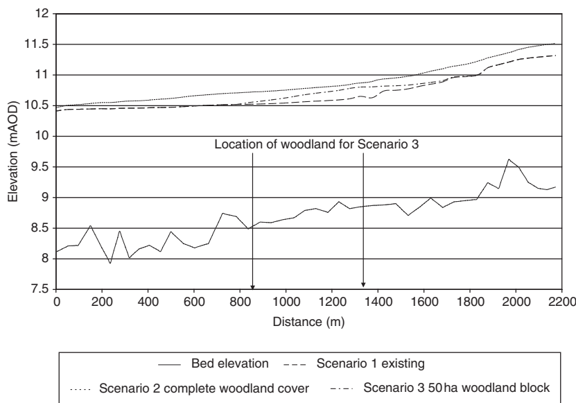
Fig. 4. Longitudinal profile displaying water and bed levels along the modelled reach, as well as the location of the wooded area in Scenario 3. mAOD, metres above ordnance datum.
