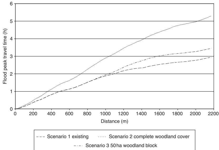
Fig. 8. Average travel time of the flood peak along the modelled reach.
