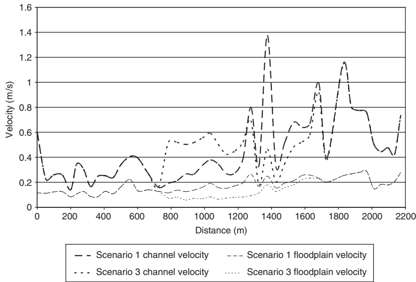
Fig. 7. Comparison of water velocity profiles for the main channel and the wooded north bank of the floodplain.
