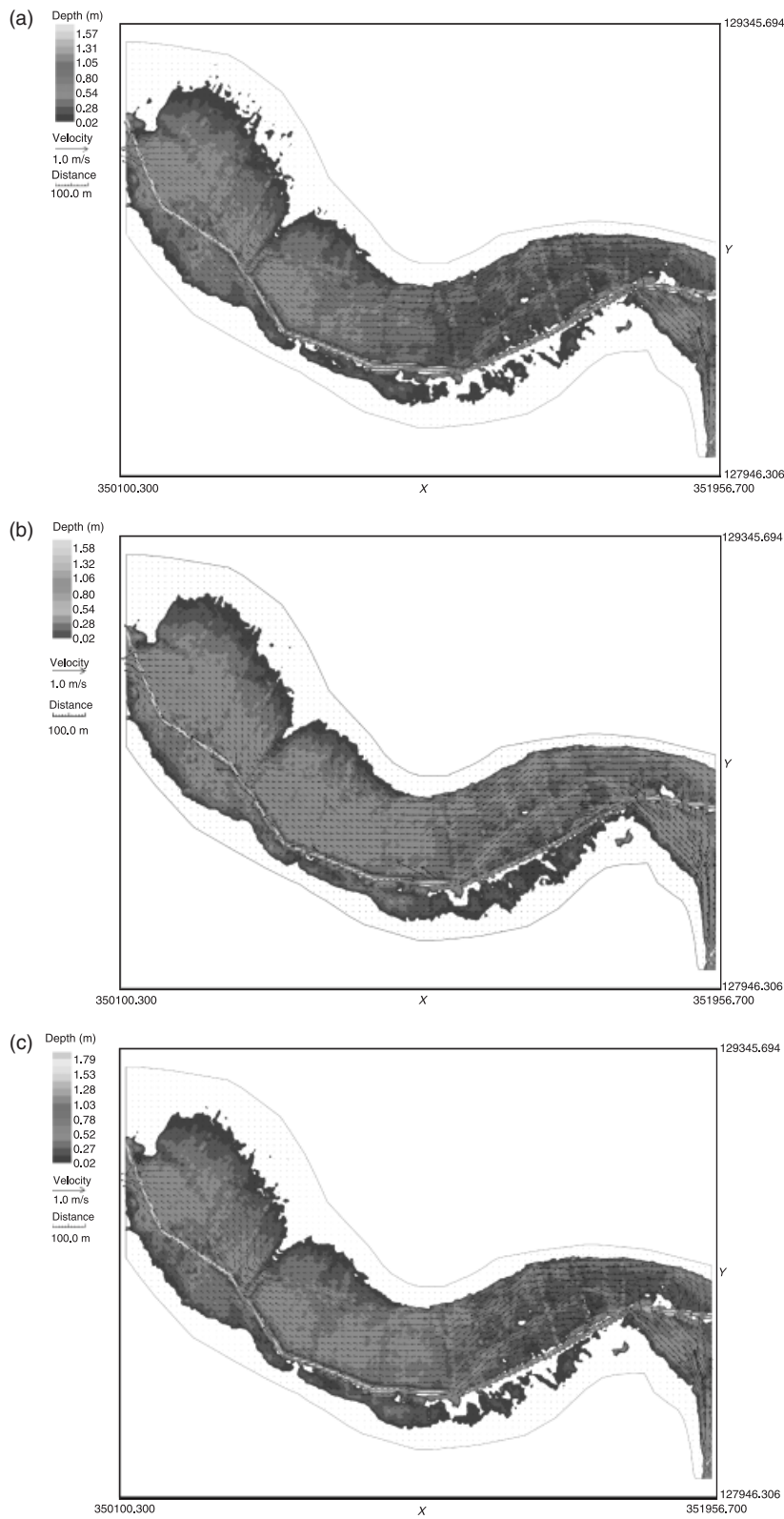
Fig. 9. (a) Flood depth and flow velocity assuming the floodplain is covered by pasture (Scenario 1). Arrow length is proportional to velocity. (b) Flood depth and flow velocity for a complete cover of floodplain woodland on the north bank of the floodplain (Scenario 2). Arrow length is proportional to velocity. (c) Flood depth and velocity for a central block of woodland over the whole width of the floodplain (Scenario 3: area of woodland outlined in black). Arrow length is proportional to velocity.
