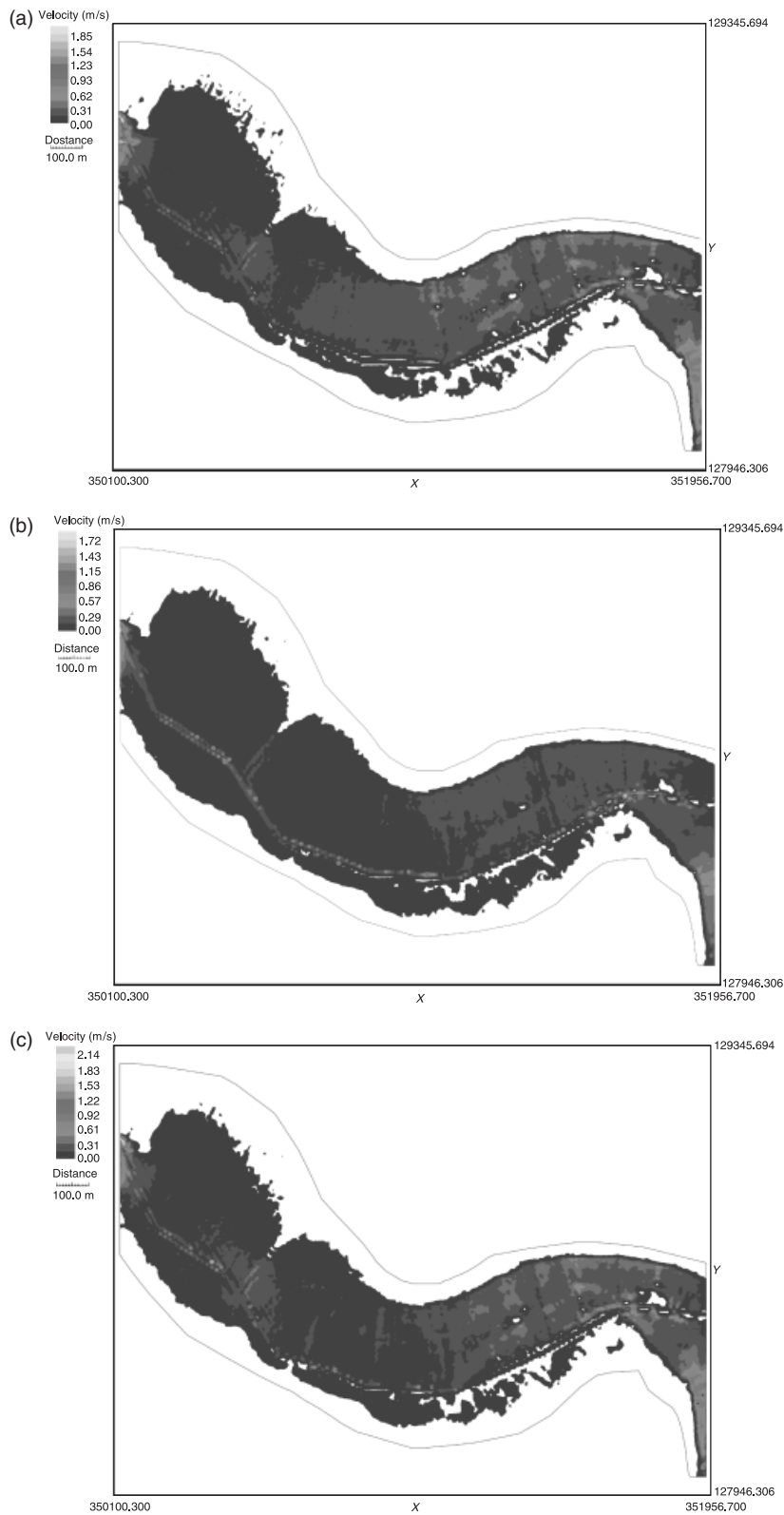
Fig. 10. (a) Flow velocity map for a floodplain covered with pasture (Scenario 1). (b) Flow velocity map for a complete cover of floodplain woodland on the north bank of the floodplain (Scenario 2). (c) Flow velocity map for a central block of floodplain woodland extending over the whole width of the floodplain (Scenario 3: area of woodland outlined in black).
