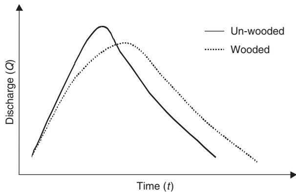
Fig. 1. Theoretical time discharge hydrograph showing the possible effect of floodplain woodland on flood flows ( Q , discharge; t , time).
