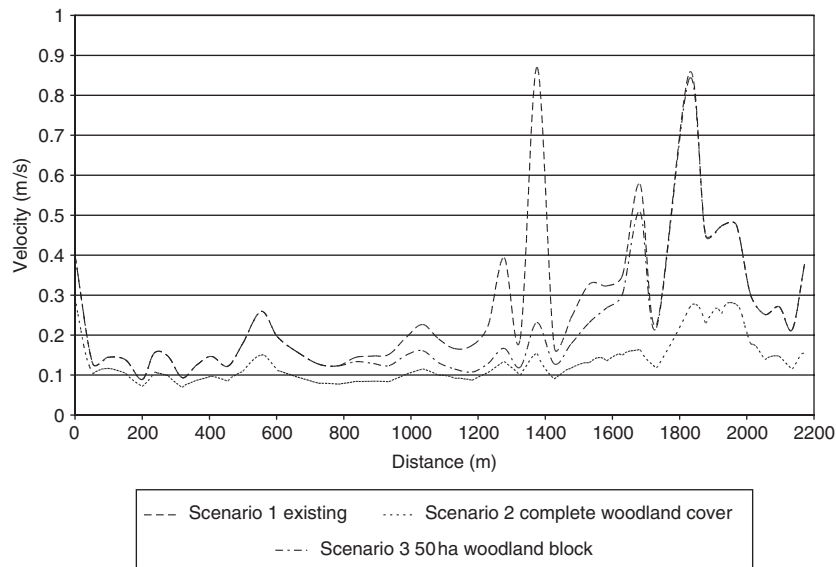
Fig. 6. Average water velocity profile along the modelled reach.
