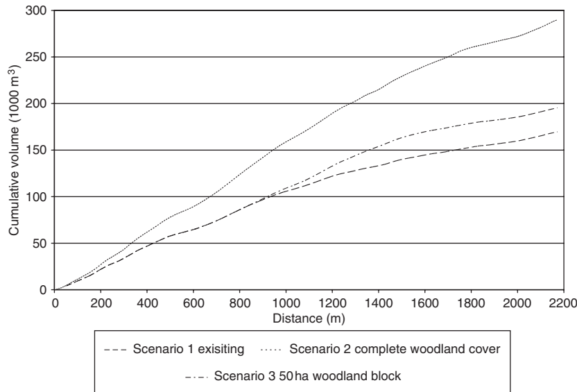
Fig. 5. Flood storage volume with distance along the modelled reach.
