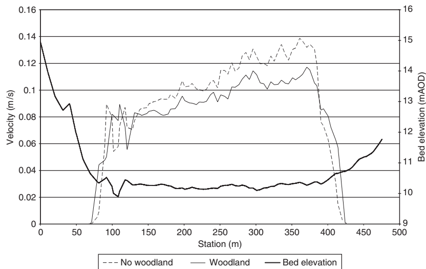
Fig. 11. Cross section of floodplain and channel comparing changes in velocity for non-wooded (Scenario 1) and partly wooded (Scenario 3) scenarios.
