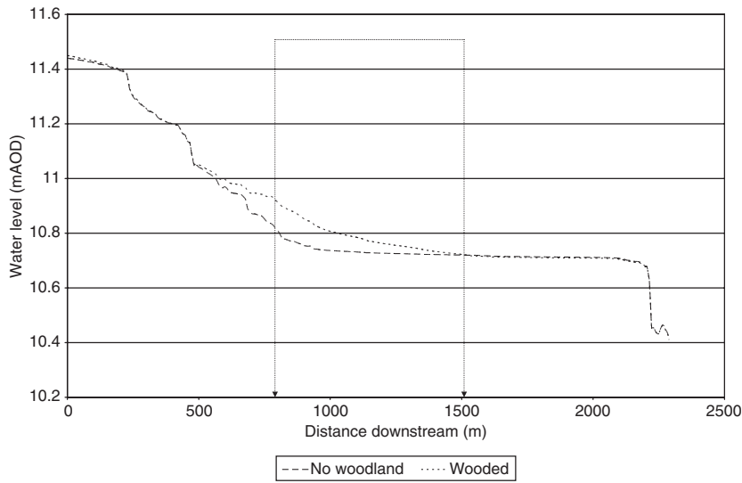
Fig. 12. Longitudinal water surface profile along a section of modelled river reach (arrows define limits of woodland in Scenario 3). mAOD, metres above ordnance datum.
