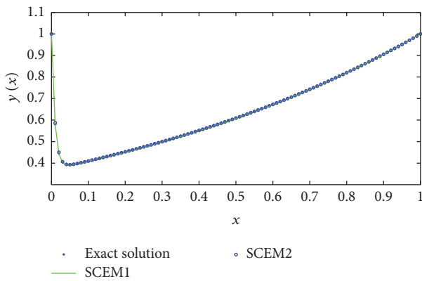
FIGURE 1: Left layer problem for \epsilon = 0.01 and \delta = 0.1\epsilon .
