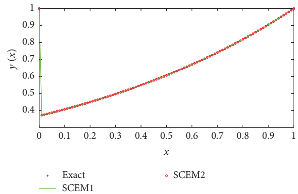
FIGURE 3: Left layer problem for \epsilon = 0.001 and \delta = 0.9\epsilon .
