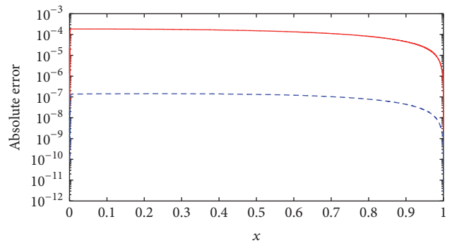
FIGURE 3: Left layer problem for \epsilon = 0.001 and \delta = 0.9\epsilon .
