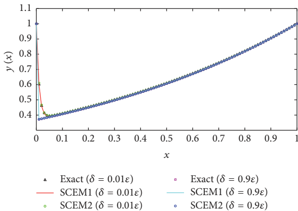
FIGURE 2: Delay effect on left layer problem for \epsilon = 0.01 , \delta = 0.01\epsilon , and \delta = 0.9\epsilon .
