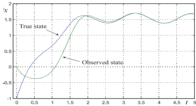
Fig. 3. True and observed variable {}^1x in the case of \bar{x} = -1 .
