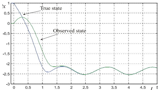
Fig. 1. True and observed variable {}^1x in the case of \bar{x} = 1 .
