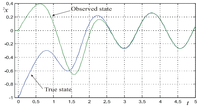
Fig. 4. True and observed variable {}^2x in the case of \bar{x} = -1 .
