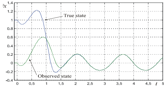
Fig. 2. True and observed variable {}^2x in the case of \bar{x} = 1 .
