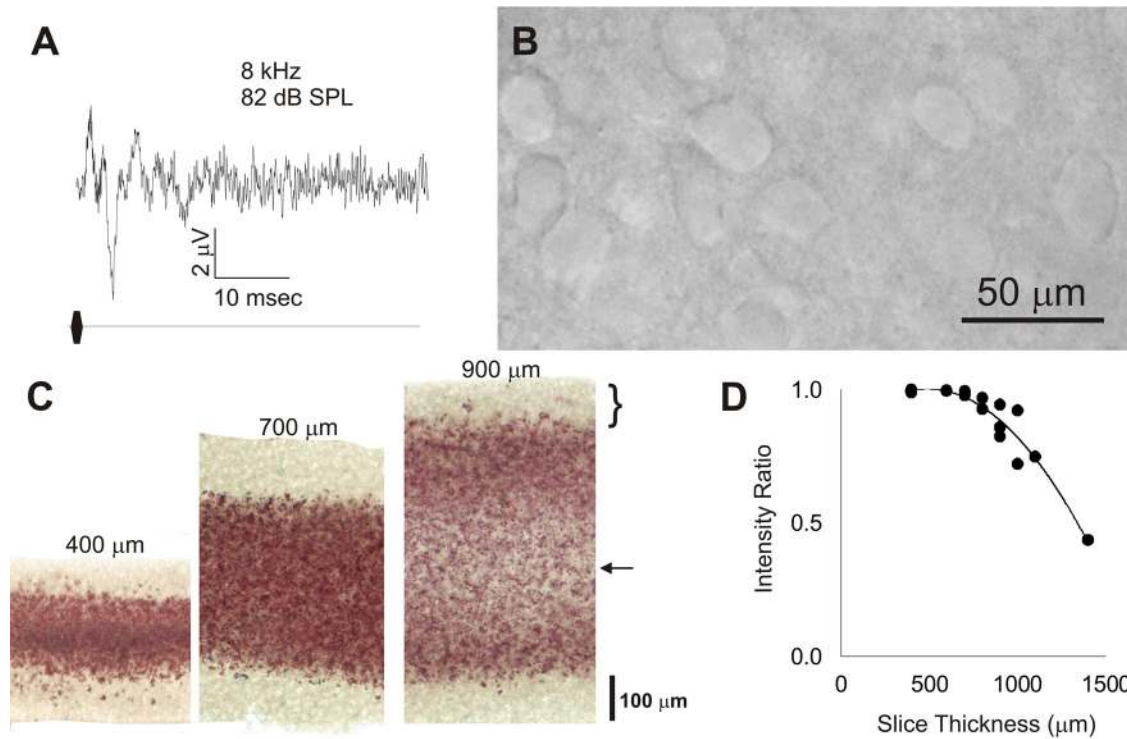
Fig. 2. A : auditory brain-stem response taken from a mouse pup at postnatal day 12 , taken as an average of 1,000 trials. SPL, sound-pressure level. B : differential interference contrast image from the cerebral cortex of a 600- \mu\text{m} thick slice \sim 4 h after slicing. C : 2,3,5-triphenyltetrazolium chloride (TTC)-stained slices obtained from slices cut at 400, 700, and 900 \mu\text{m} . Bracket corresponds to pale area on the perimeter of all of the slices corresponding to poor TTC signal. Arrow corresponds to the pale area in the interior of the 900- \mu\text{m} slice, suggesting poor viability in this portion of the thick slice. D : plot of the ratio of TTC staining intensity in the center of the slice vs. peak intensity just deep to the surface vs. thickness. Data were pooled from 6 different animals. Equation for fit curve: y = -7\text{E}-07x^2 + 0.0007x + 0.8364 , r^2 = 0.92 .
