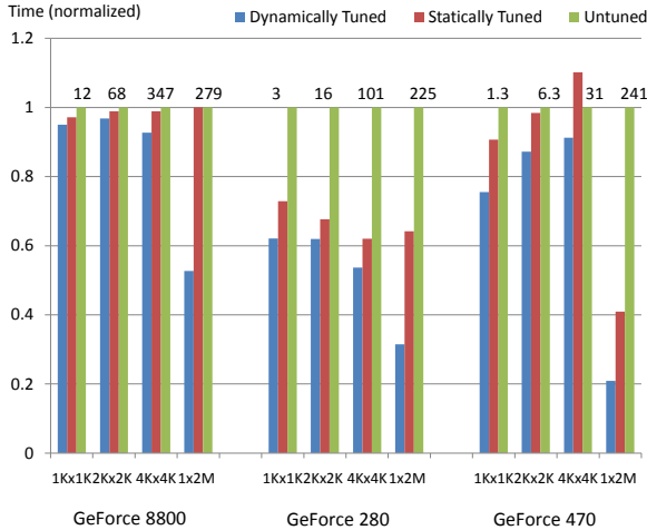
Figure 7: Comparison of non-tuned, statically tuned, and dynamically tuned performance for various workloads and GPUs. 1K×1K stands for 1024 1024-equation systems and 1×2M stands for 1 system of 2 million equations. The timings are normalized to the untuned (or default parameters) execution time. The numbers on top of the columns indicate the non-tuned execution time in milliseconds.
